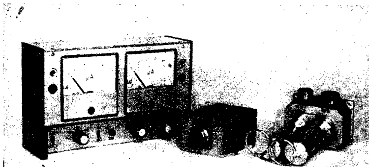
Optical photometer OF 71 for the study of the composition of the upper atmospheric layers of the earth. Used on Interkosmos 11 and 16 satellites.
