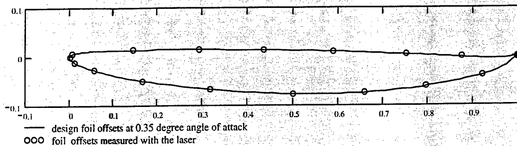
Figure 4-2: Laser Varification of Foil Angle of Attack
