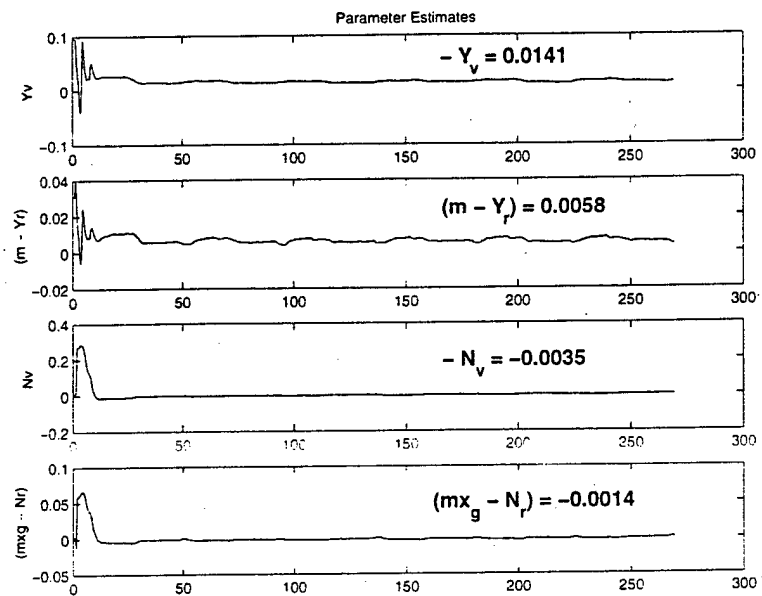
Figure 4-2: Parameter Estimates Using the Rudder Model from [43]
