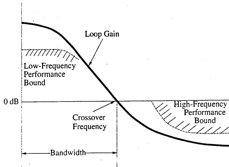
Figure 5-1: The Goal of Loopshaping
