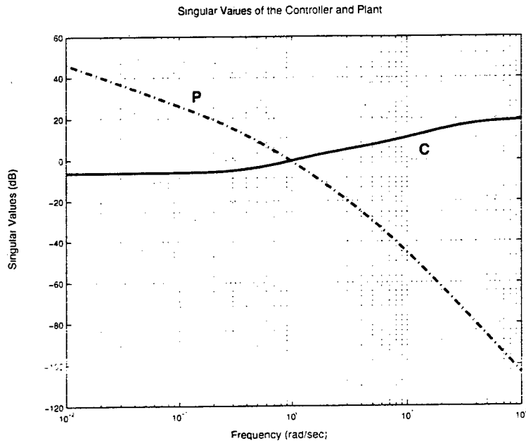
Figure 5-10: Plant and Controller Open-Loop Gains
