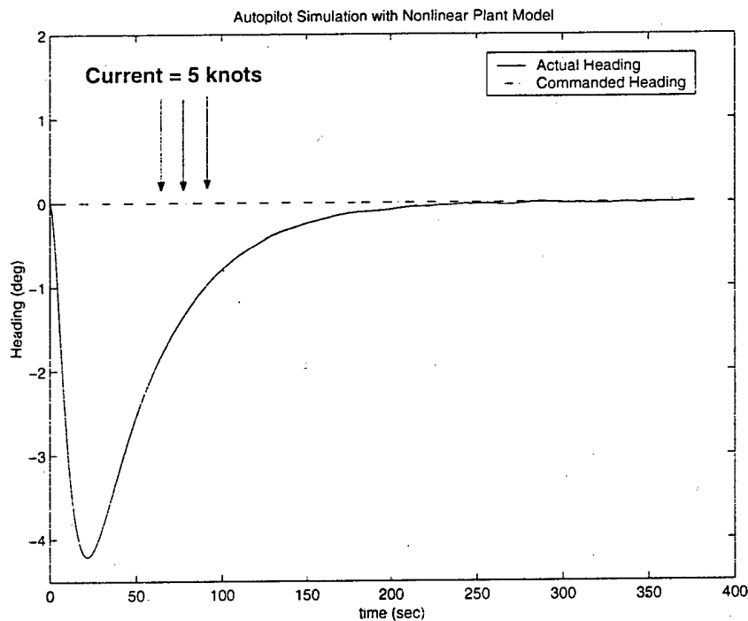
Figure 5-8: Nonlinear Plant Heading Change During Current Rejection
