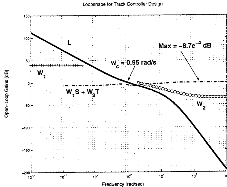
Figure 5-15: Loopshape for Cross-Track Error Controller Design
