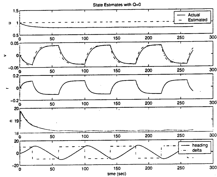
Figure 4-4: State Estimates During a 10^\circ/10^\circ Zig-Zag Maneuver with Q=0
