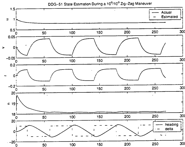
Figure 4-8: State Estimates During a 10^\circ/10^\circ Zig-Zag Maneuver
