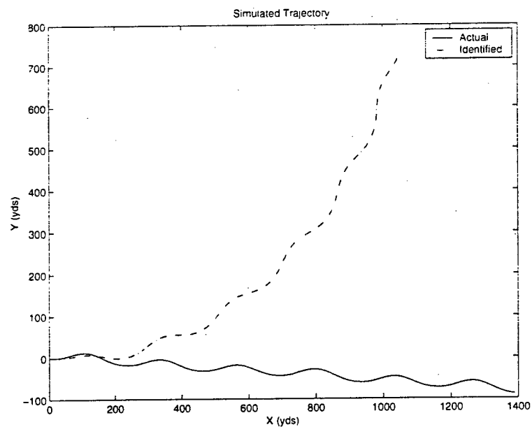
Figure 4-3: Trajectory Simulation Using the Rudder Model from [43]
