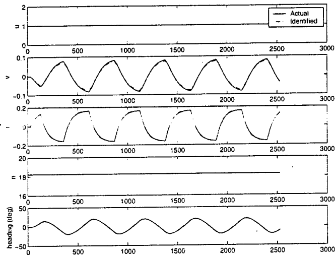
Figure 2-5: Simulated States of the Esso Osaka During a 10^\circ/10^\circ Zig-Zag Maneuver
