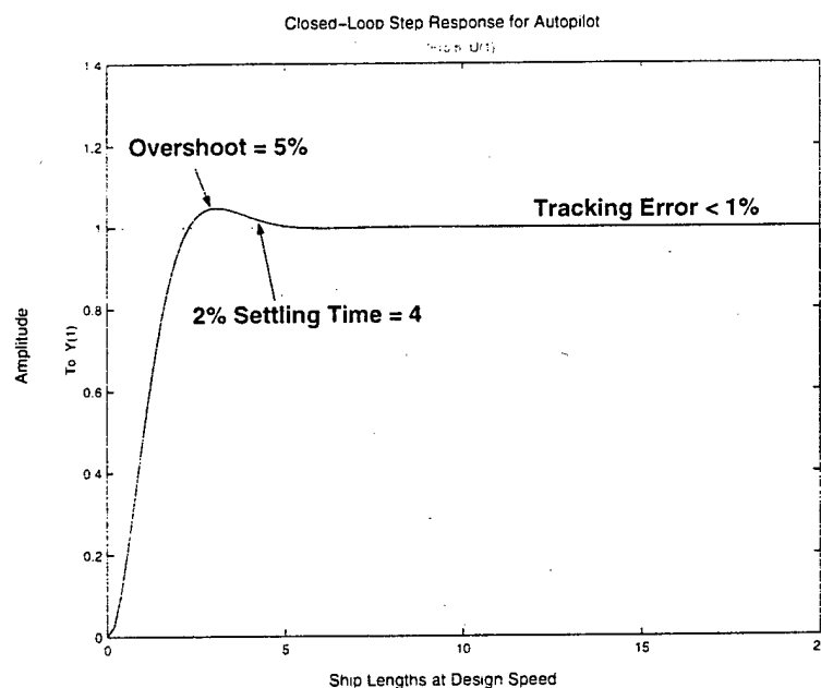
Figure 5-6: Closed-Loop Autopilot Step Response
