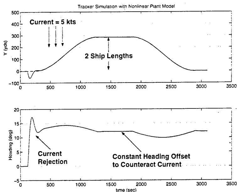
Figure 5-18: Trajectory and Heading during Nonlinear Plant Simulation
