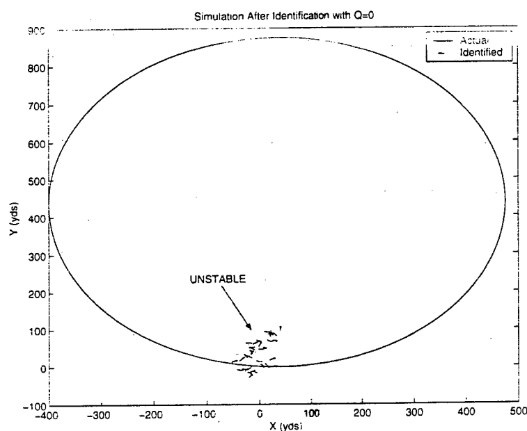
Figure 4-6: Simulation of a 10° Rudder Steady Turn with Q=0
