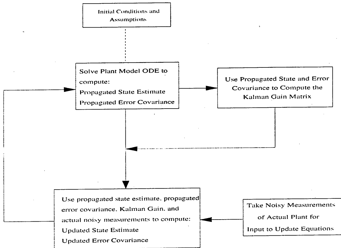
Figure 2-1: EKF Algorithm Flowchart
