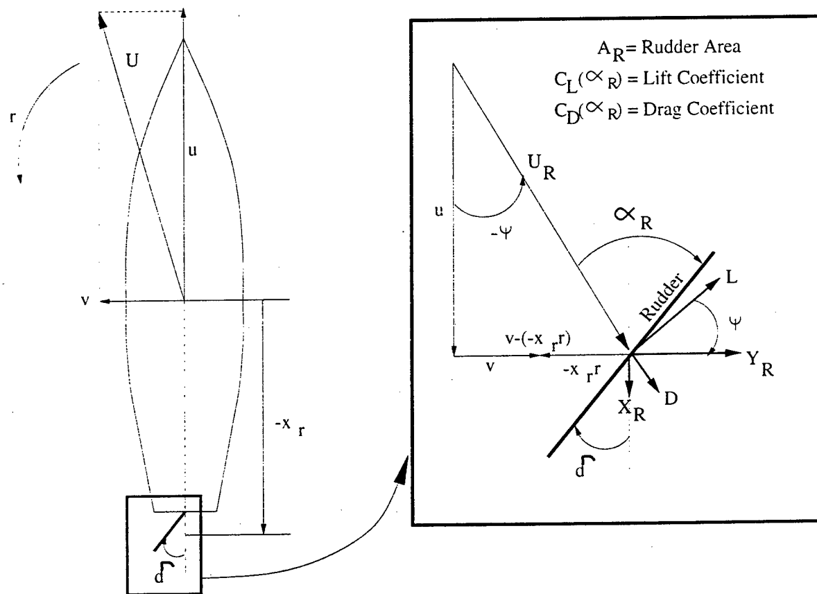
Figure 3-2: Vector Diagram of Rudder Forces
