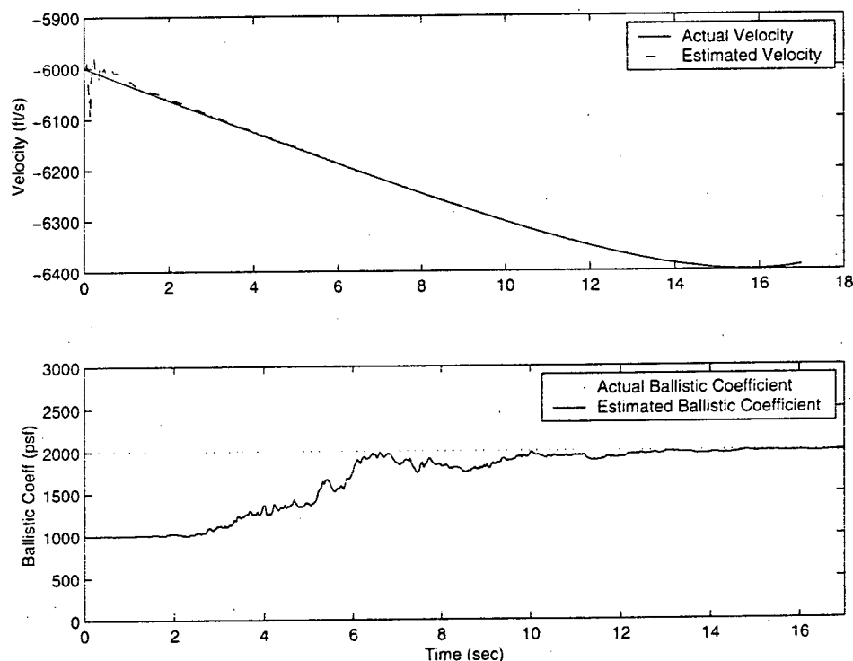
Figure A-2: EKF Application
