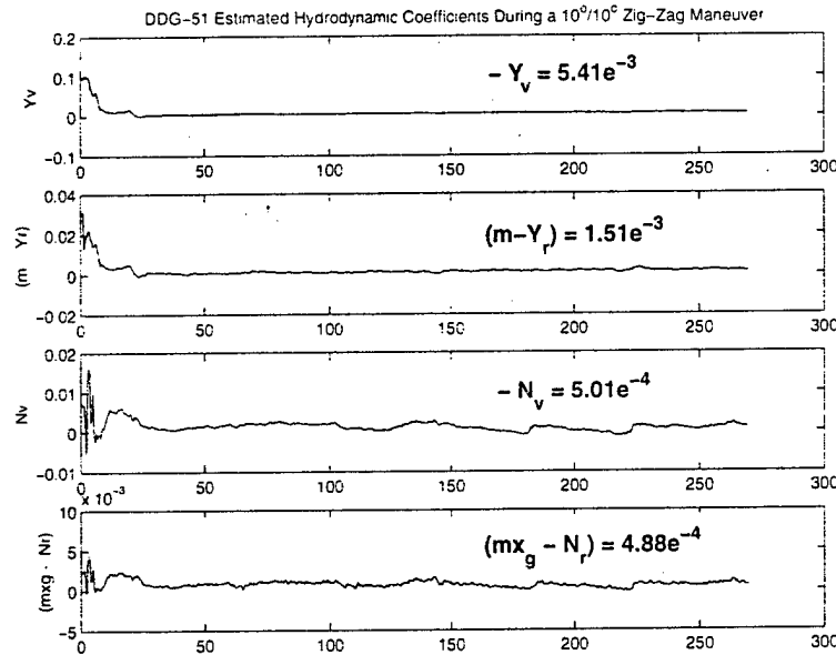
Figure 4-9: Parameter Estimates During a 10^\circ/10^\circ Zig-Zag Maneuver
