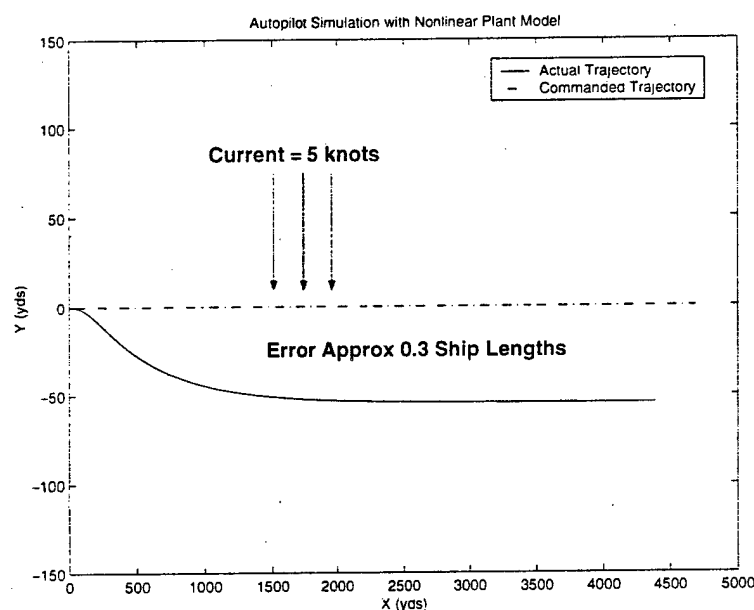
Figure 5-7: Nonlinear Plant Trajectory During Current Rejection
