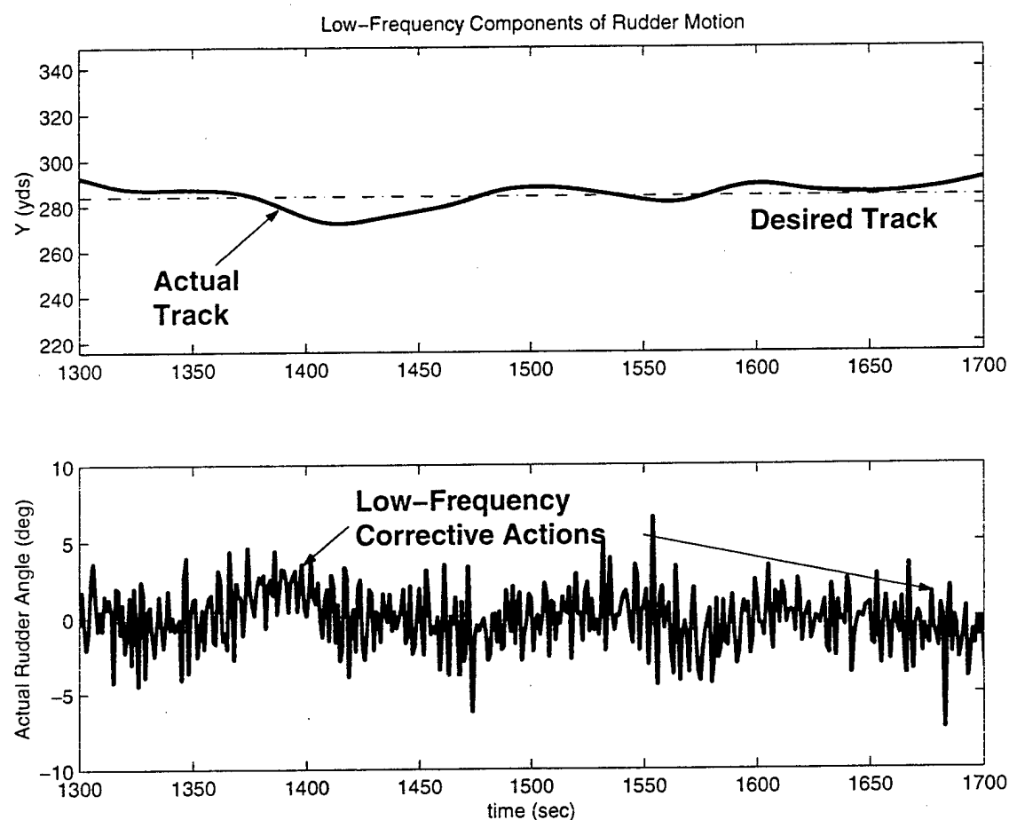
Figure 5-24: Low-Frequency Component of Actual Rudder Angles
