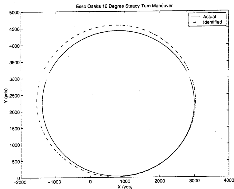
Figure 2-7: Simulated Trajectory of the Esso Osaka During a 10^\circ Rudder Steady Turn
