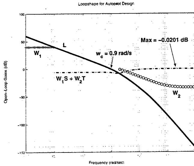
Figure 5-4: Loopshape for Autopilot Design
