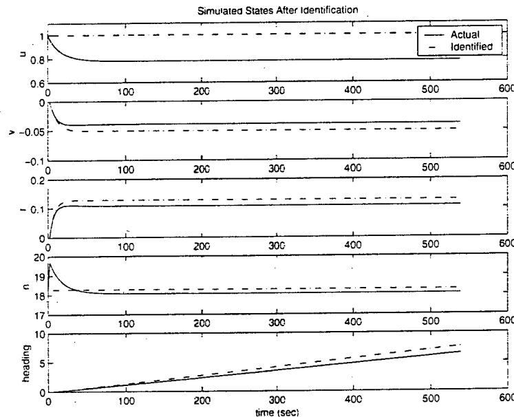
Figure 4-10: Simulated States During a 10° Rudder Steady Turn
