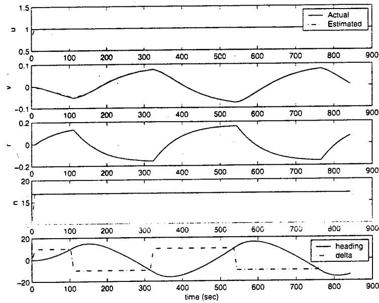
Figure 2-3: State Estimates of the Esso Osaka During a 10^\circ/10^\circ Zig-Zag Maneuver
