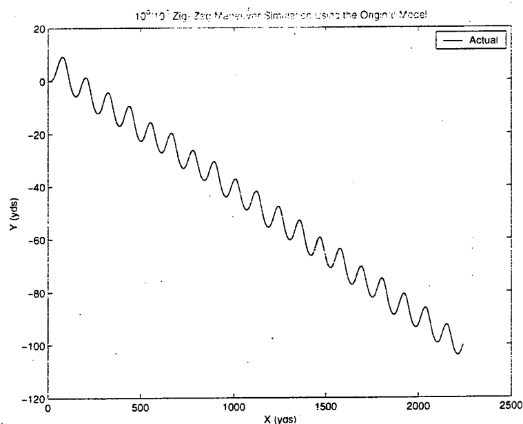
Figure 4-1: 10°/10° Zig-Zag Maneuver Using the Rudder Model in [43]
