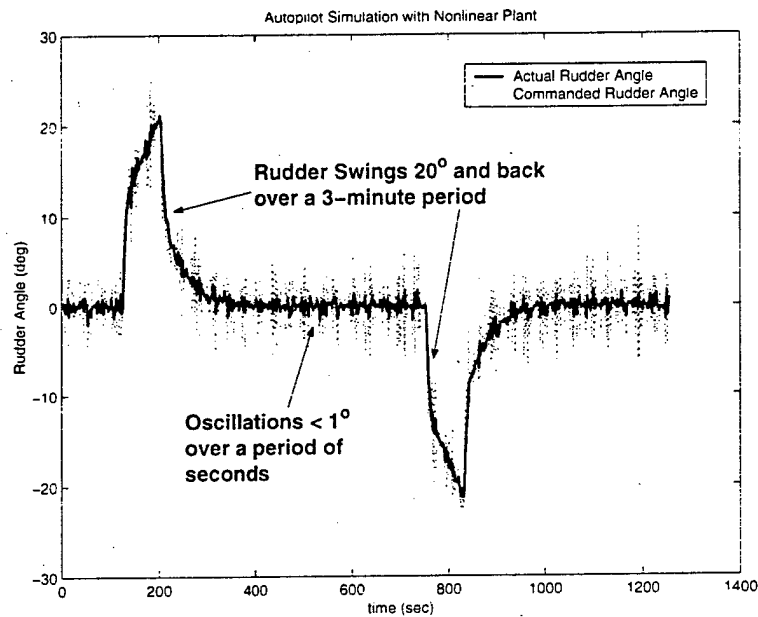
Figure 5-13: Actual and Commanded Rudder Angle During Track-Changing Maneuver
