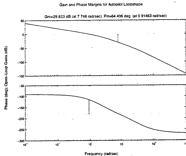
Figure 5-5: Gain and Phase Margins for Autopilot Design
