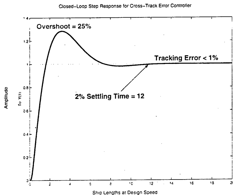
Figure 5-17: Cross-Track Error Controller Closed-Loop Step Response
