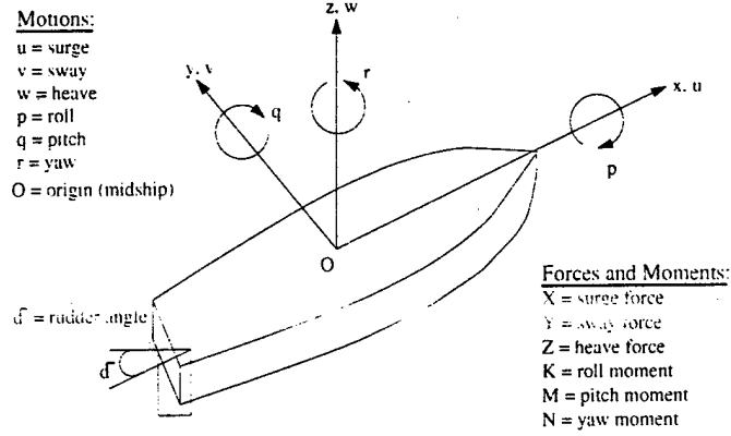
Figure 3-1: Body-Fixed Coordinate System
