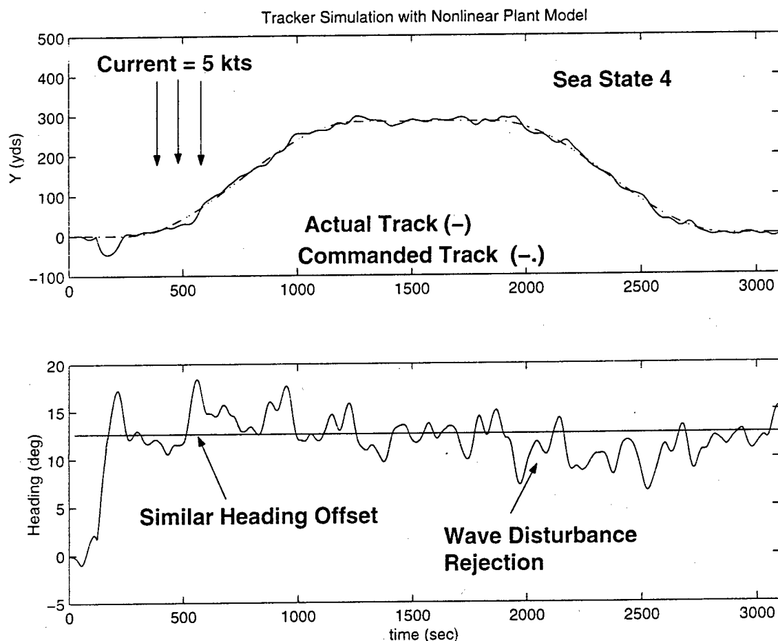
Figure 5-22: Trajectory and Heading During Track Change
