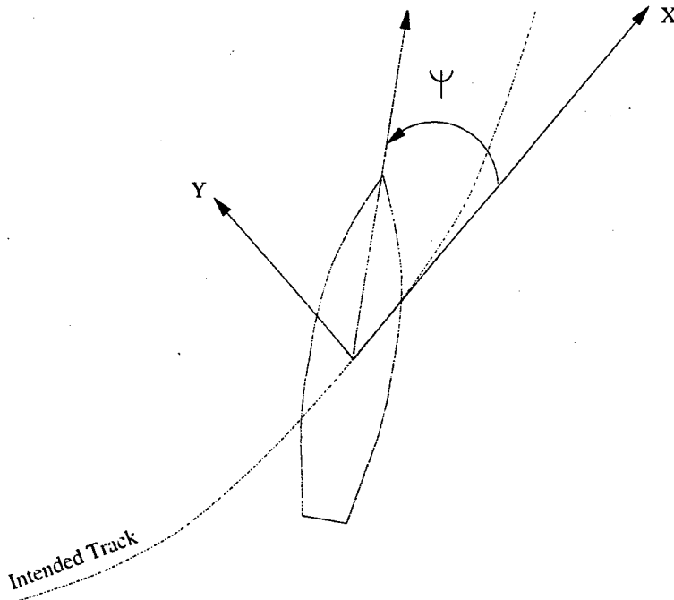
Figure 5-14: New Coordinate System for Track Controller
