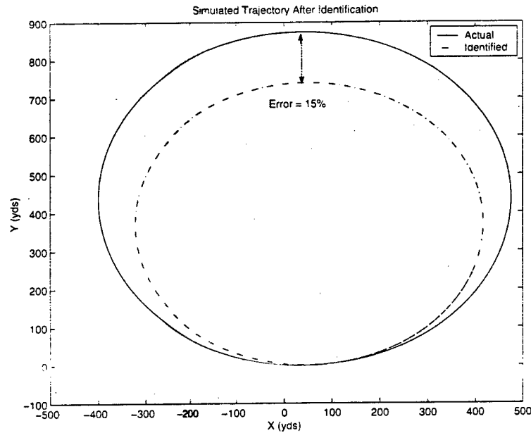
Figure 4-11: Simulated Trajectory During a 10^\circ Rudder Steady Turn
