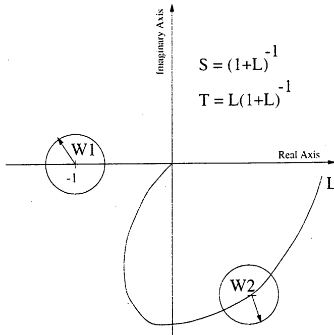
Figure 5-3: Nyquist Plot of Performance Specifications
