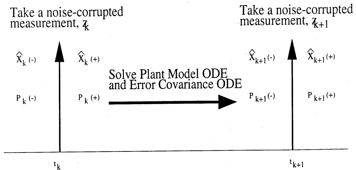
Figure 2-2: EKF Timing Diagram Adapted from Figure 4.2-1 of [19]
