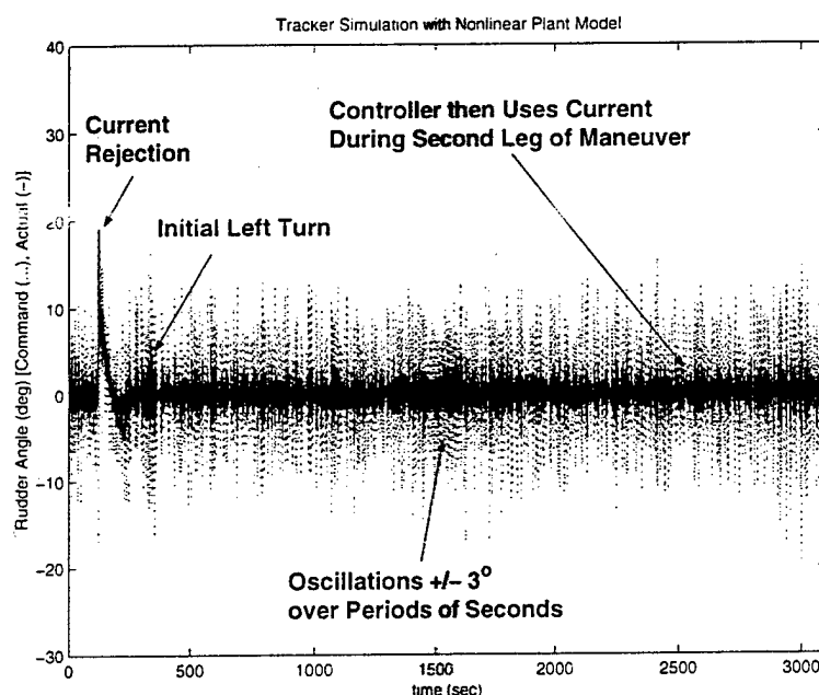
Figure 5-19: Actual and Commanded Rudder Angle During Nonlinear Plant Simulation
