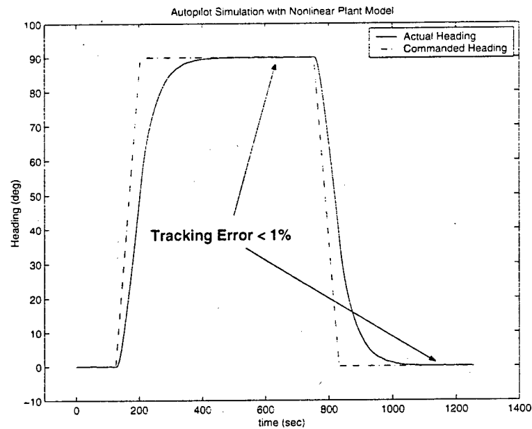
Figure 5-12: Nonlinear Plant Heading Angle during Track-Changing Maneuver with Autopilot
