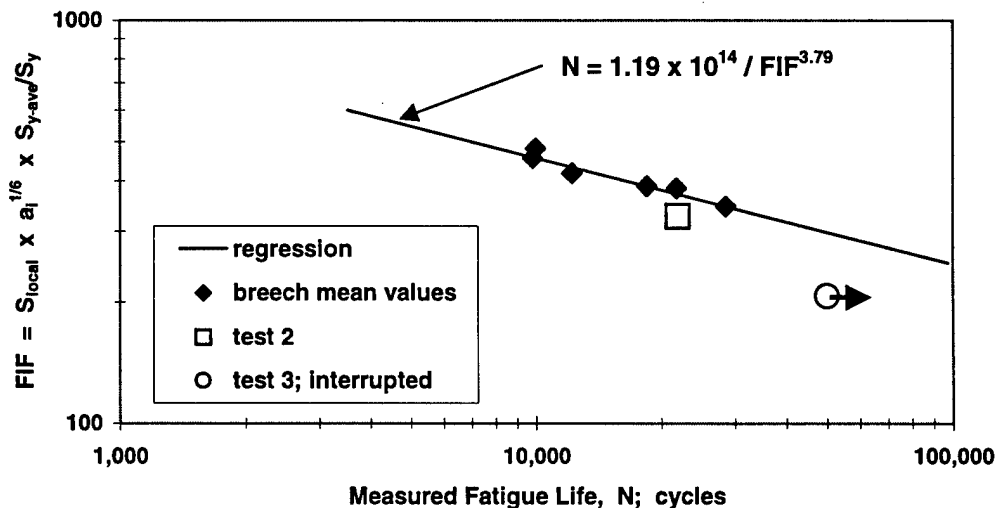
Figure 4. Comparison of two recent tests with mean lives from cannon breach tests.
