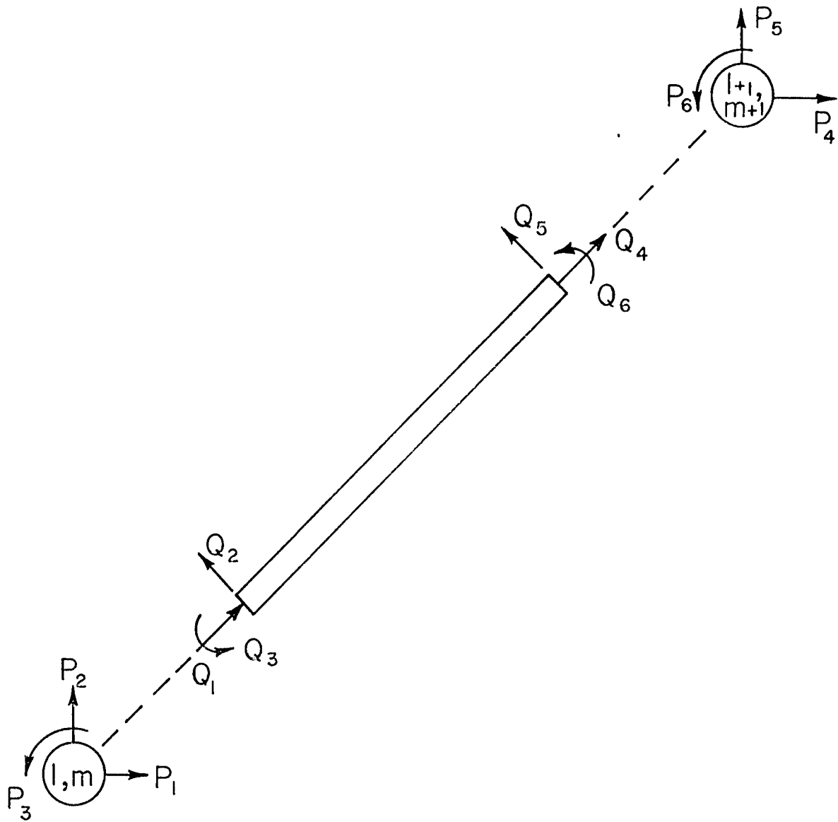
Figure 5. Beam Element Connecting Lattice Points (l, m) and (l+1, m+1) .
