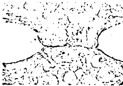
Figure 5. Welding of matrix foils with collision point located at the center between the fibers (fiber: V2A 0.1 mm; matrix: nickel 0.1 mm)
