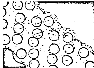
Figure 33. Inconel-718 matrix with tungsten fibers, annealed 96 hrs. at 1100° C.
