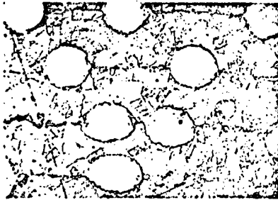
Figure 30. Nickel matrix with V2A fibers, annealed for 9 hrs. at 800° C.
