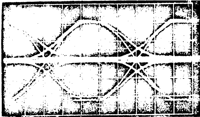
Figure 5. Oscilloscope of "decision-making eyes" at the point of decision-making of the repeater for a length of the cable sector of 800 meters, diameter 0.8 millimeter of Cu, t = 100 ns/division, U = 1 V/division.
