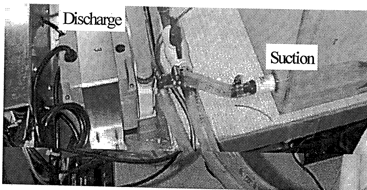
Figure 7. De-ballast Pump
