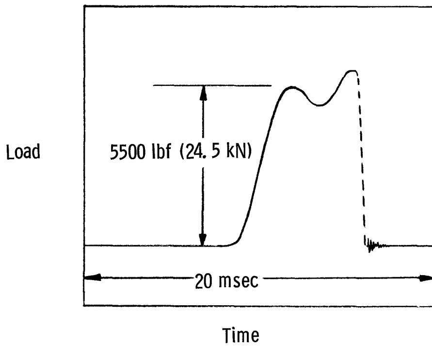
Figure 4.- Representative load time history for transverse Ti-4Al-3Mo-1V notched specimen at a strain rate of 5.0 per second.
