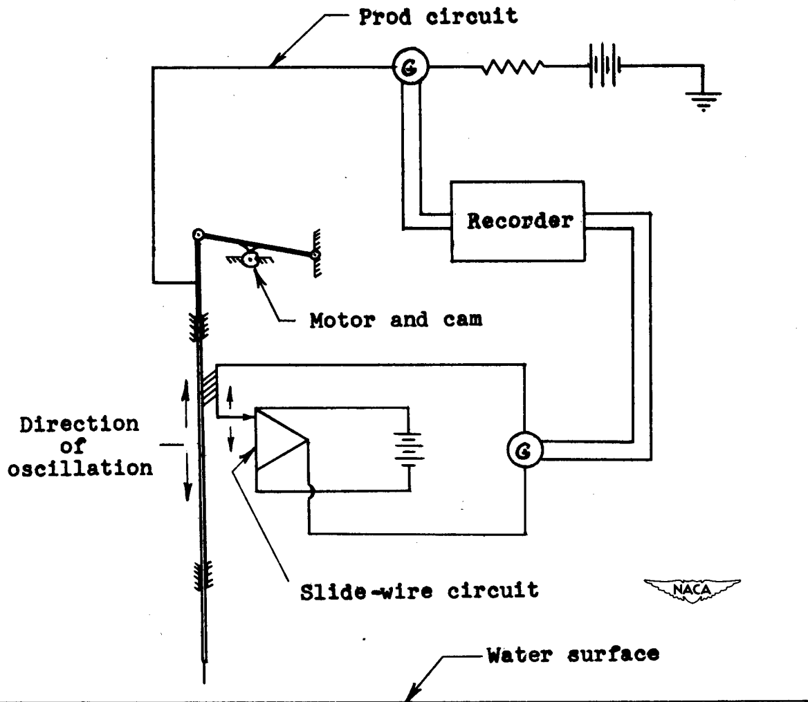
Figure 4.- Schematic drawing of water-level recorder.
