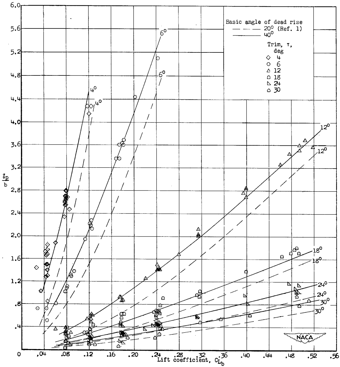
Figure 8.- Variation of nondimensional center-of-pressure location with lift coefficient.
