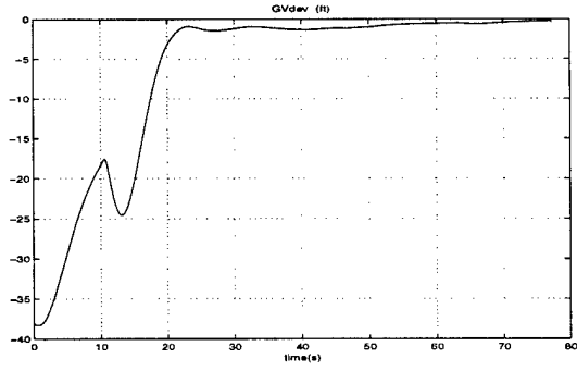
Figure 29: Vertical Deviation from Gliding Path
