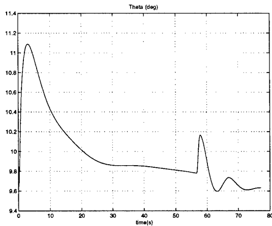
Figure 22: Pitch Evolution During Switching Experiment
