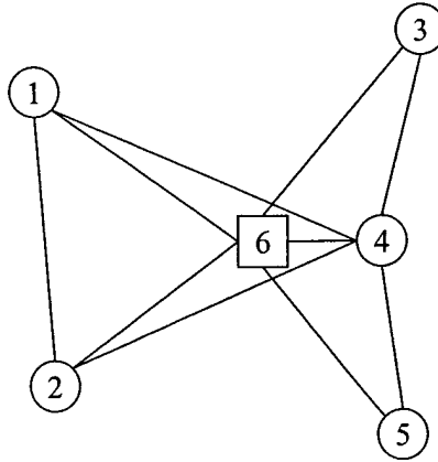
Figure 5-7: Single-hub network for demonstrating the strength of ESSND , RO , and ARM coefficient reduction thereby removing some of this fractionality. In RO , however, this absorption is accomplished only on individual aircraft routes whose capacity exceeds one of its gateway-hub demands. When individual aircraft routes do not cover their gateway-hub demands, we create composite variables to cover these demands. The process of combining routes may, however, result in excess capacity, which we can absorb by reducing the capacity-demand coefficients and reduce the fractionality even further.
