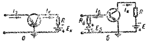
Fig.1. Switching circuit:
