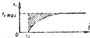
Fig. 9. Curve of Ion Current Growth.
