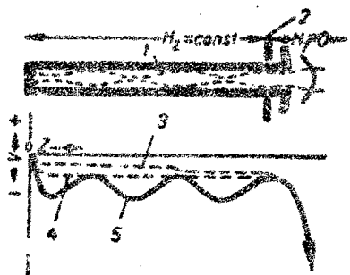
Fig.5. Distribution of potential in length of beam focused by magnetic field: 1 - beam; 2 - magnetic screen; 3 - potential at axis with \rho = -10^{-6} mm of mercury column; 4 - potential at the axis with \rho = \sim 10^{-8} mm of mercury column; 5 - potential at axis in the absence of ions.
