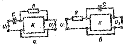
Fig.1. Basic circuit diagram of connection of a passive RC circuit and an electronic amplifier:
