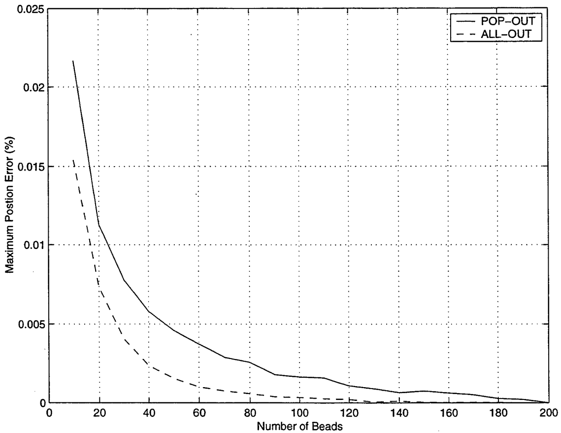
Figure 4. Maximum Position Error of Follower.
