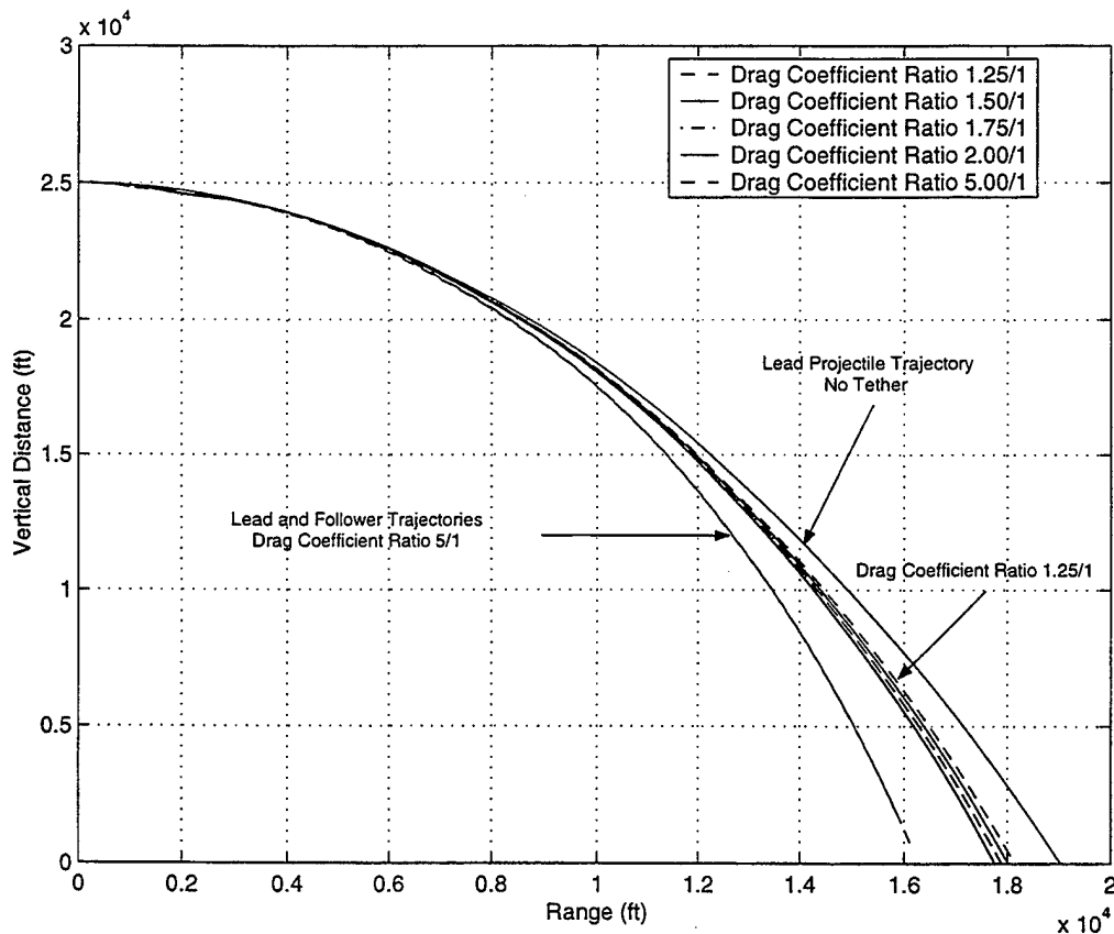
Figure 9. Range of Lead and Follower (Lead/Follower Mass Ratio 1%).
