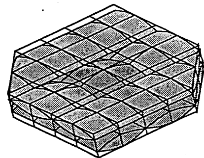
Unit cell
