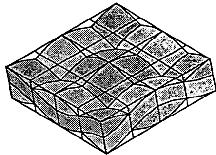
Unit cell
