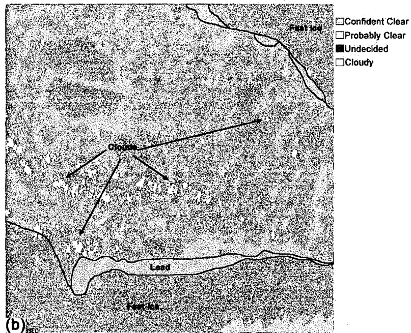
NPS Cloud Mask
