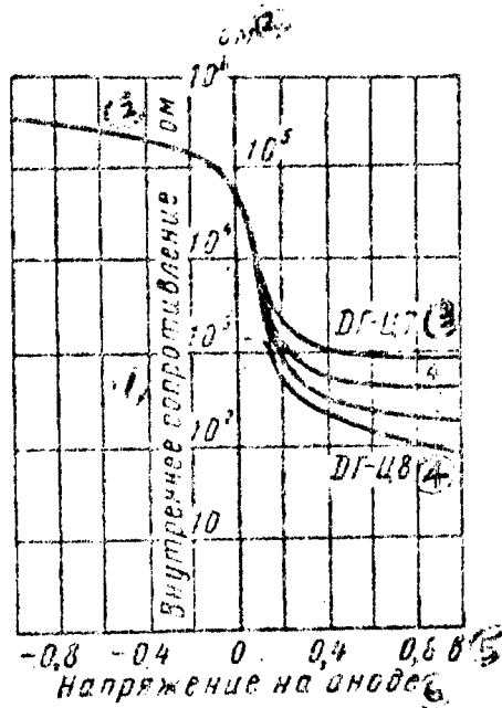
Figure 6. Internal resistance of point-contact germanium diodes DG-Ts.
