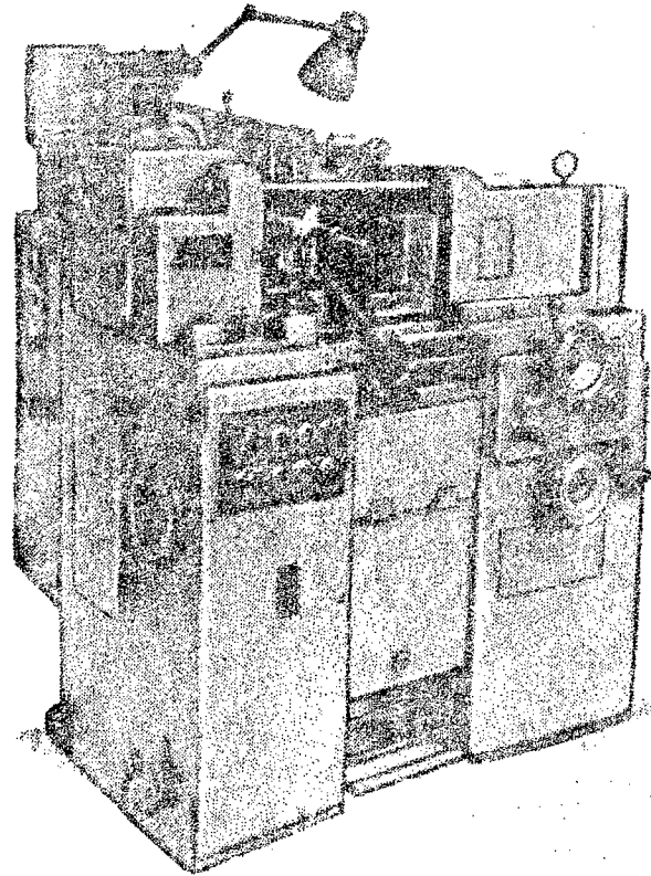
Model NR-10 automatic thread-rolling machine
