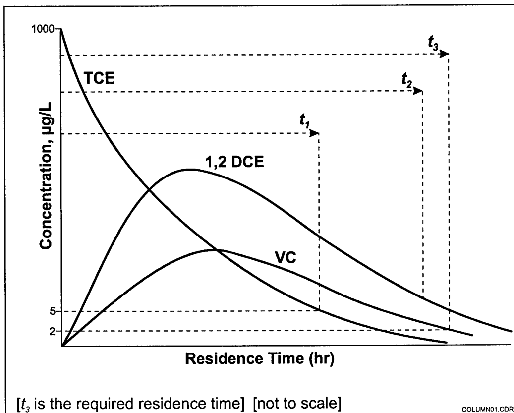
Figure 5-3. Column Concentration Profiles of TCE and Its Degradation Byproducts
