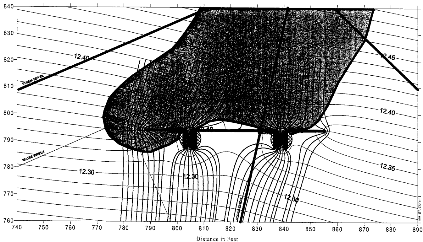
Figure 6-4. Capture Zones for the PRB at Dover AFB Showing the Effect of Fluctuating Flow Directions
