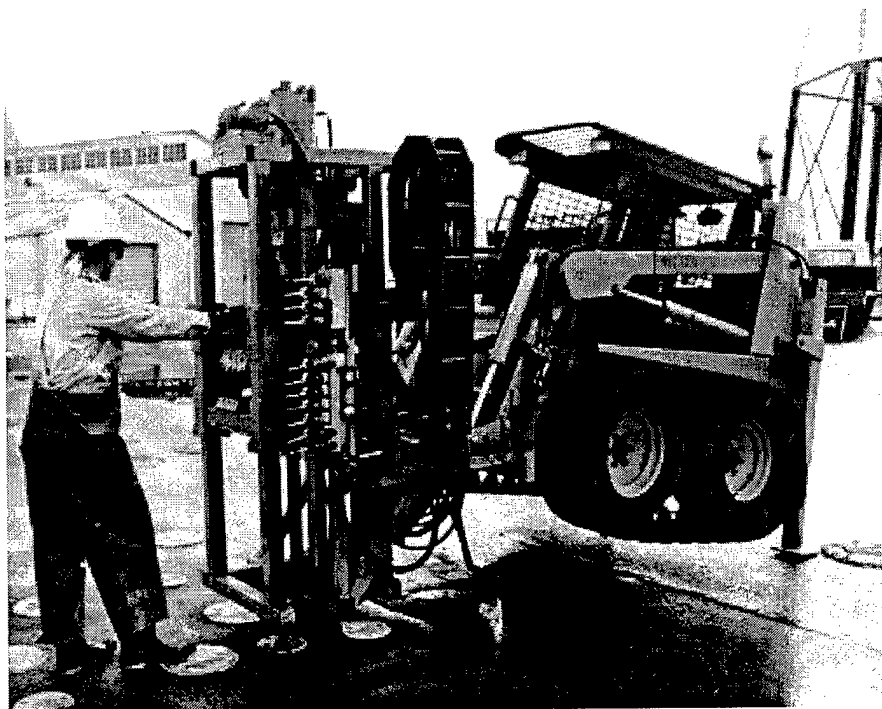
Figure 8-10. Enviro-Core™ Sampler Extracting Angled Core at Former NAS Moffett Field
