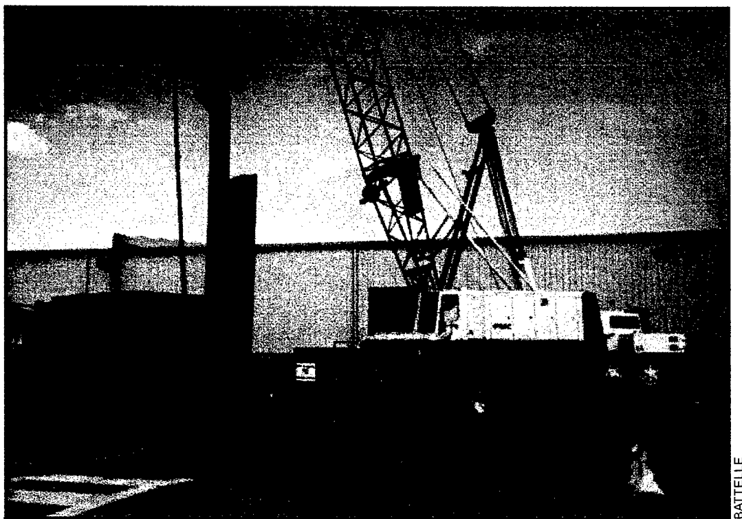
Figure 7-9. Sheet Piles Installed Using a Vibrating Hammer
