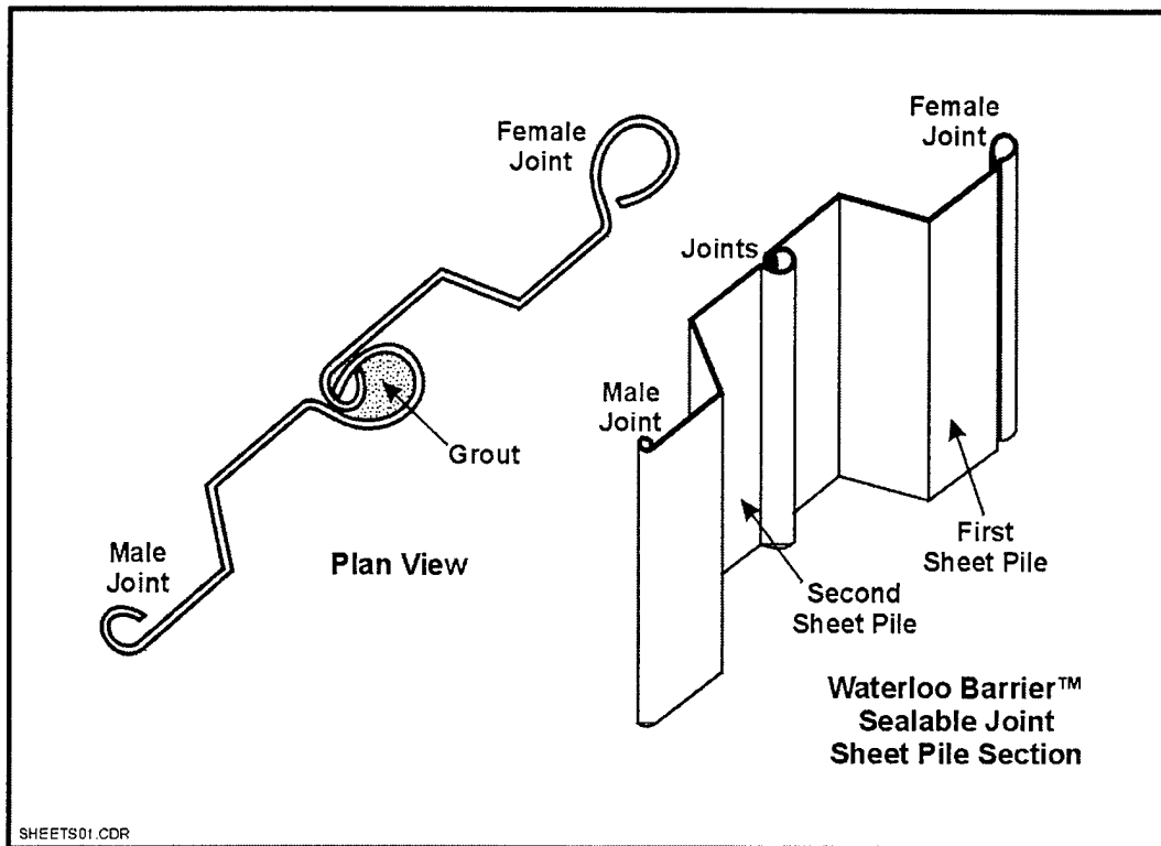
Figure 7-10. Cross Section of Sealable-Joint Sheet Piles (from Smith et al., 1995)
