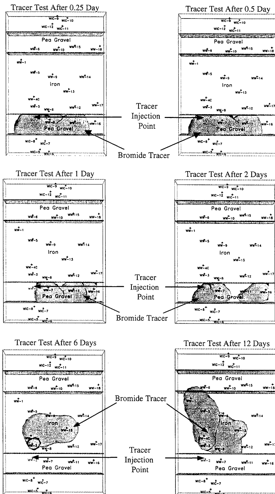
Figure 8-7. Movement of Bromide Tracer Plume through the PRB at Former NAS Moffett Field (Battelle, 1998)
