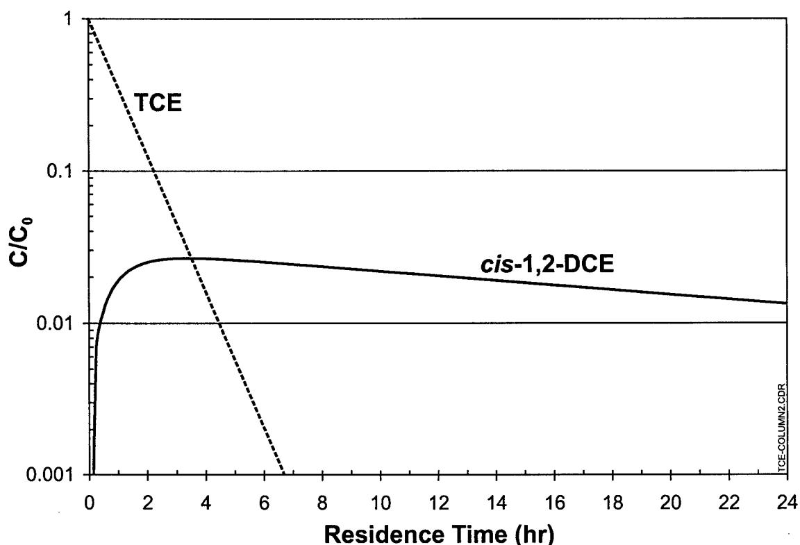
Figure 5-4. Psuedo First-Order Degradation Rate of TCE
