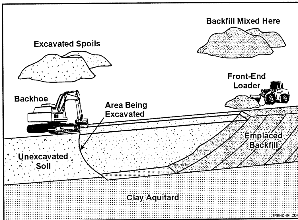
Figure 7-11. Cross Section of a Soil-Bentonite Slurry Trench, Showing Excavation and Backfilling Operations
