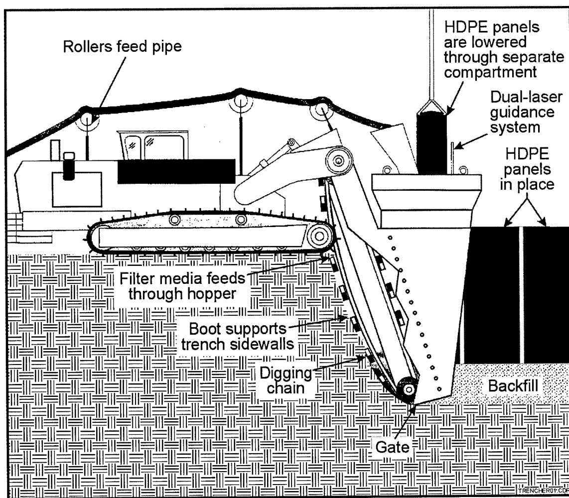
Figure 7-6. Continuous Trencher
