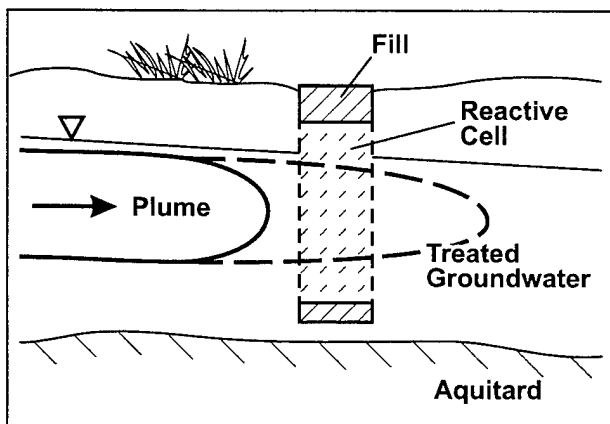
(c) Hanging barrier configuration for shallow plumes (elevation view)
