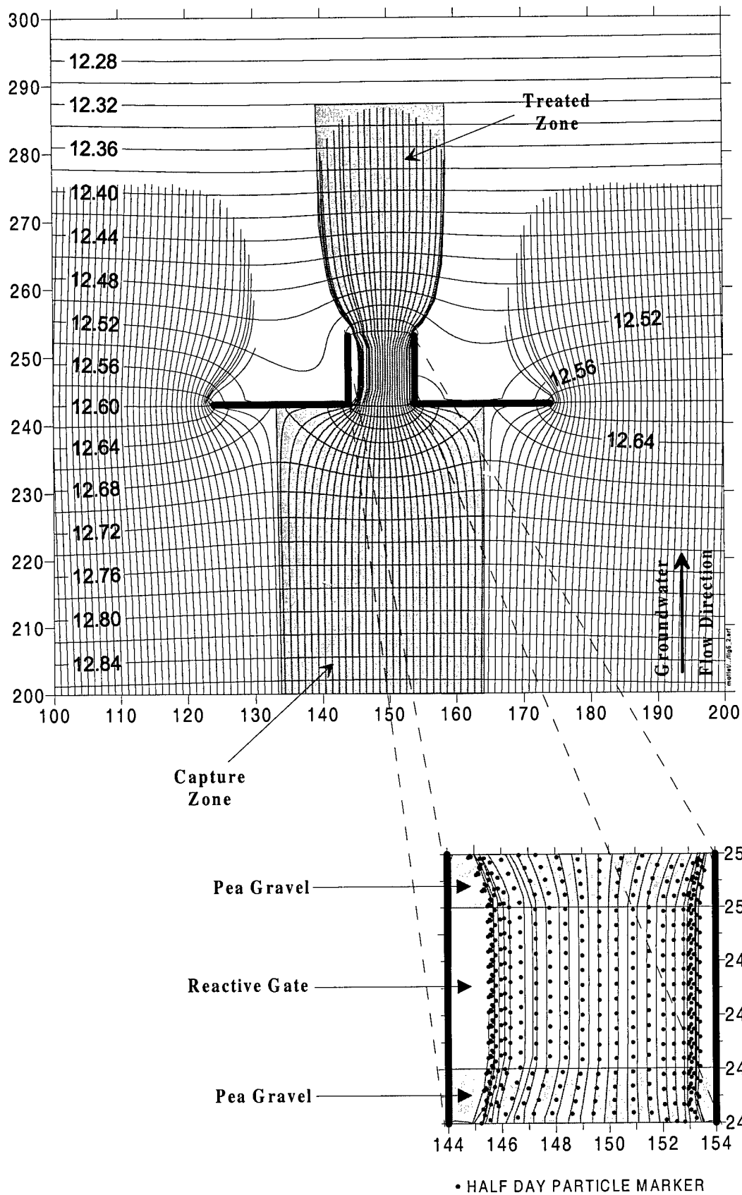
Figure 6-2. Simulated Particle Pathlines Showing Capture Zone for a Funnel-and-Gate System in a Homogeneous Aquifer
