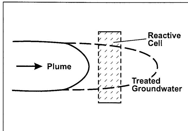
(b) Continuous reactive barrier configuration (plan view)
