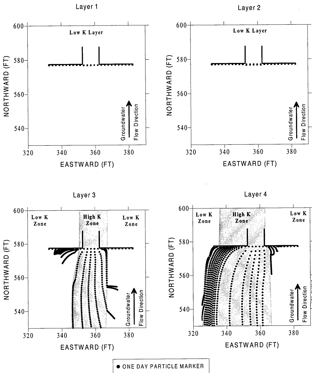
Figure 6-5. Funnel-and-Gate System at Former NAS Moffett Field Showing the Effect of Heterogeneity on Capture Zones (Battelle, 1998)
