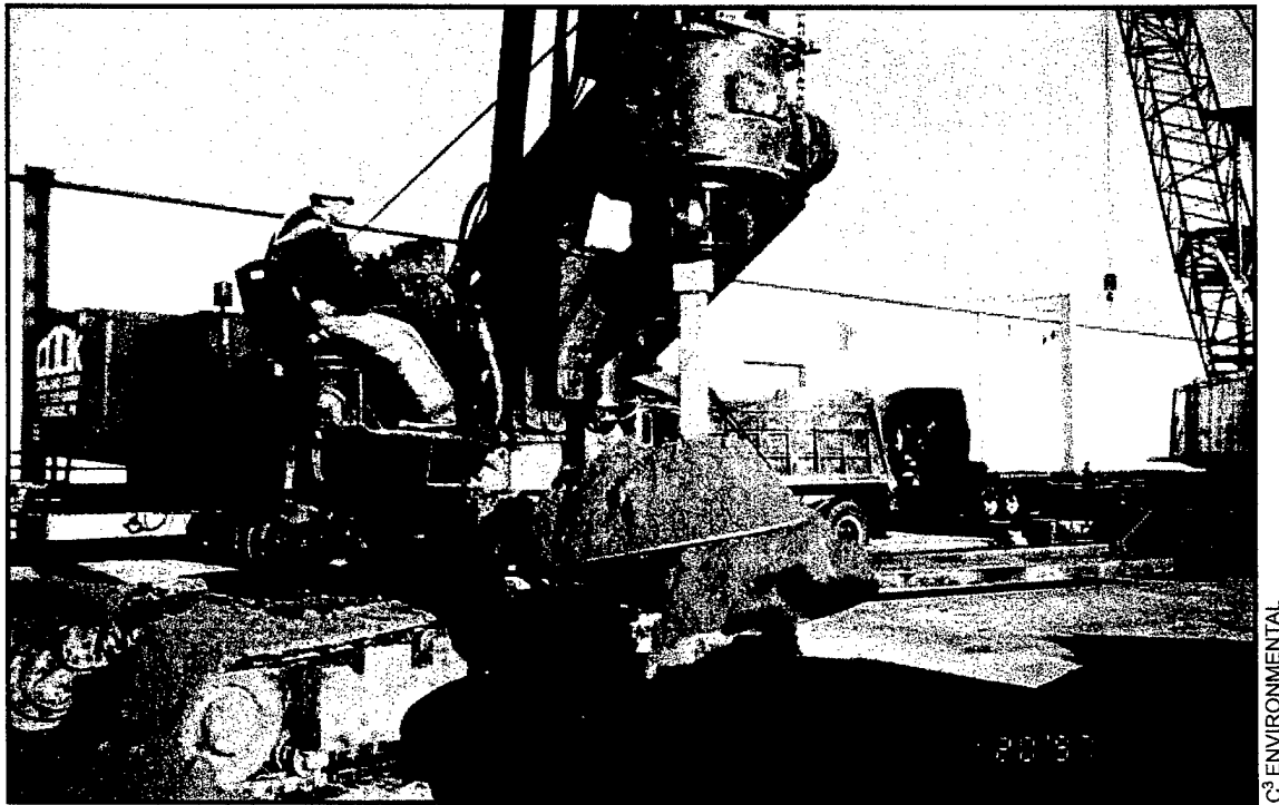
Figure 7-4. (a) Driving and (b) Excavation of a Caisson for Reactive Media Installation
