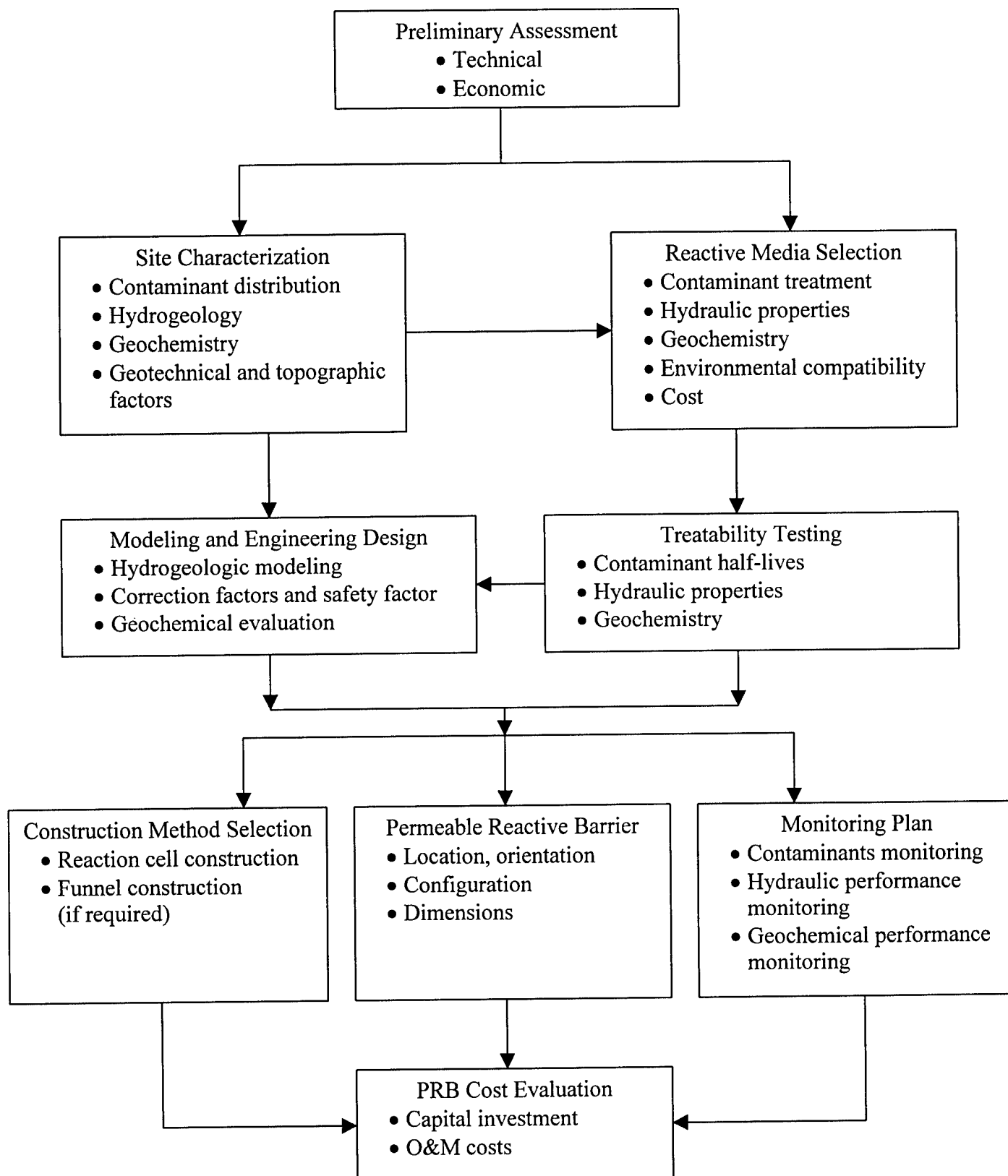
Figure 2-1. Design Methodology for a PRB Application
