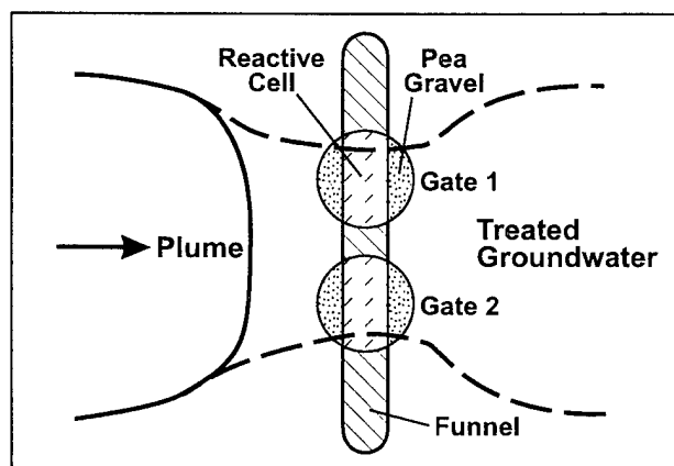
(d) Funnel-and-gate system with two gates (plan view)
