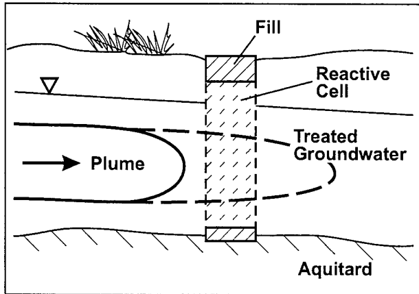
(a) PRB (elevation view)
