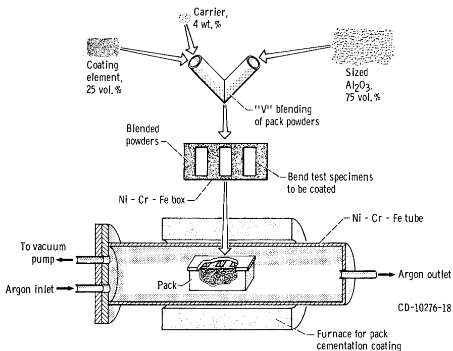
Figure 1. - Schematic of major steps involved in pack cementation process.
