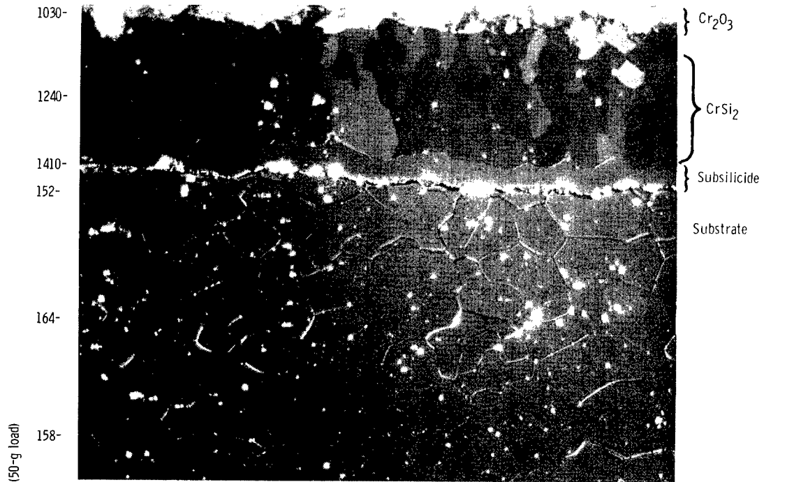
(a) Temperature, 2100° F (1420° K). Polarized light reveals columnar structure of CrSi 2 .
