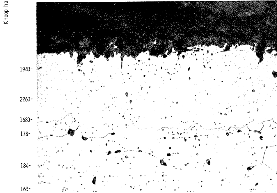
(b) Silicide coating modified with 15V - 35Mo - 35W - 15Ti, C-68-4325
