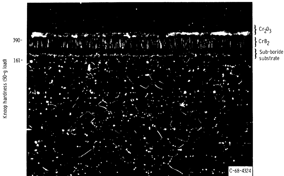
Figure 7. - Simple boride coating on Cr + 0.17 Y substrate after air exposure for 100 hours at 2100^\circ\text{F} (1420° K). Polarized light reveals columnar structure of \text{CrB}_2 . 250X.
