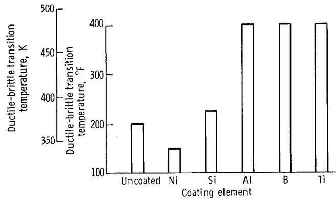
Figure 2. - Effects of simple coatings on ductile-brittle transition temperature of Cr + 0.17Y in the as-coated condition.
