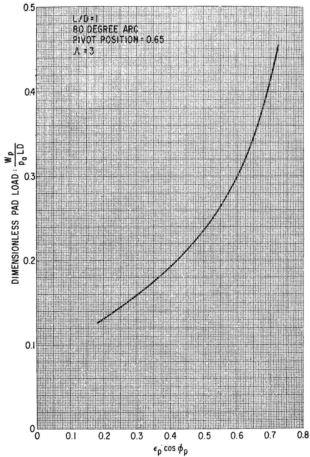
Fig. V-1 Calculated Film-Thickness Parameter versus Dimensionless Pad Load
