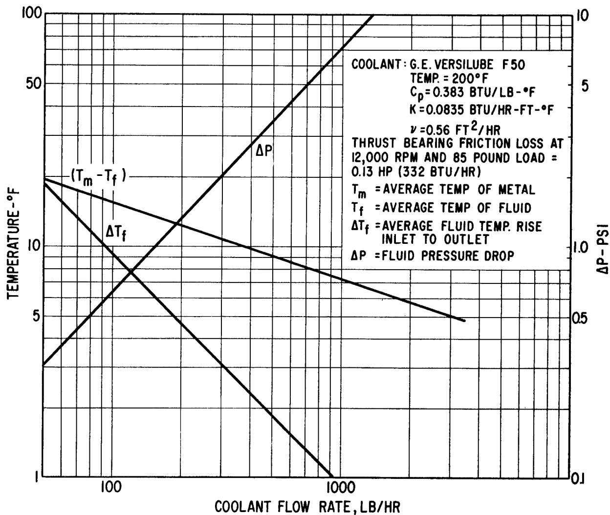
Fig. II-21 Liquid Cooled Thrust Bearing Operating Characteristics Versus Coolant Flow Rate
