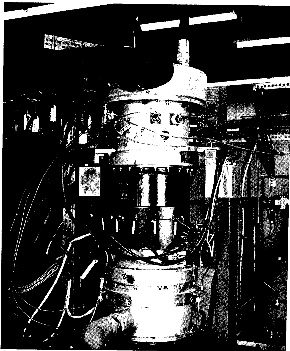
Fig. VI-7 View of Complete Simulator Installed in Vertical Position on the Test Stand
