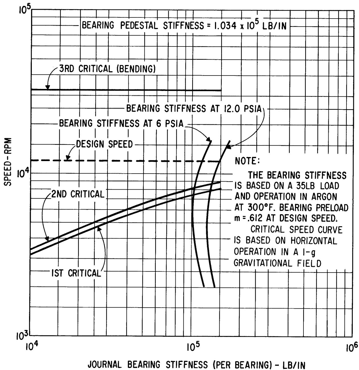
Fig. II-18 Critical Speed Versus Journal Bearing Stiffness for Turboalternator Rotor Bearing System
