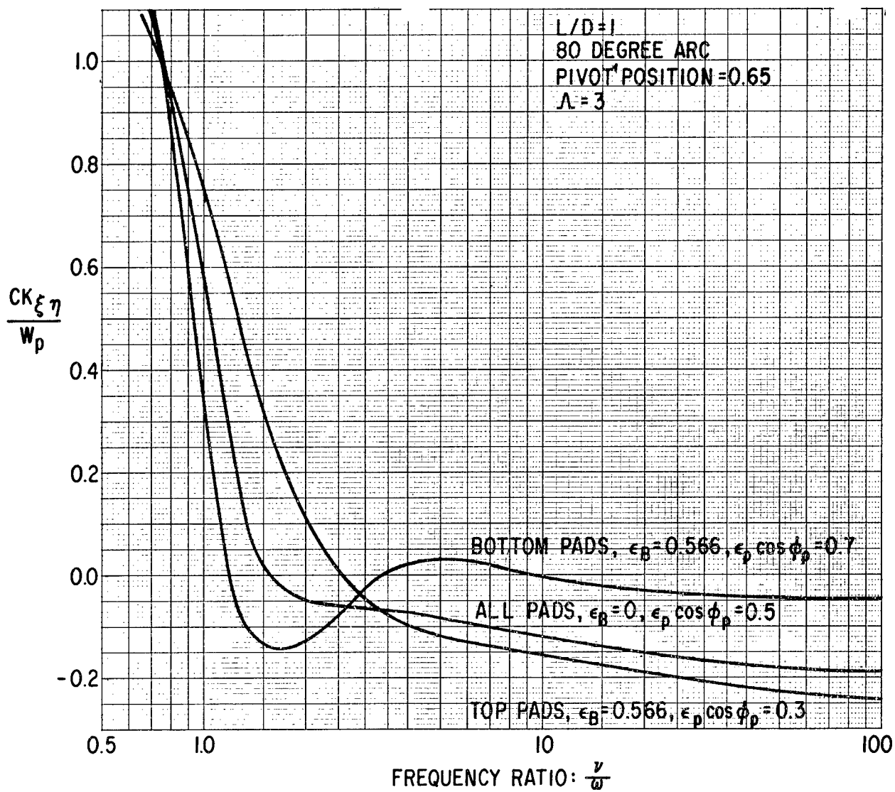
Fig. V-5 Calculated Dimensionless Pad Cross-Coupling Stiffness versus Frequency Ratio
