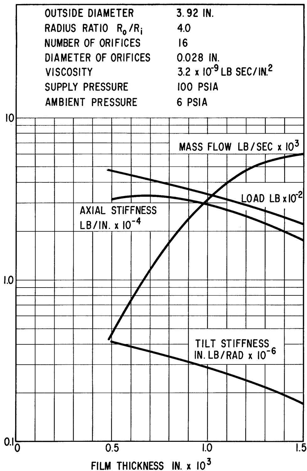
Fig. II-15 Calculated Performance of the Hydrostatic Main Thrust Bearing in a 6.0 PSIA Argon Environment
