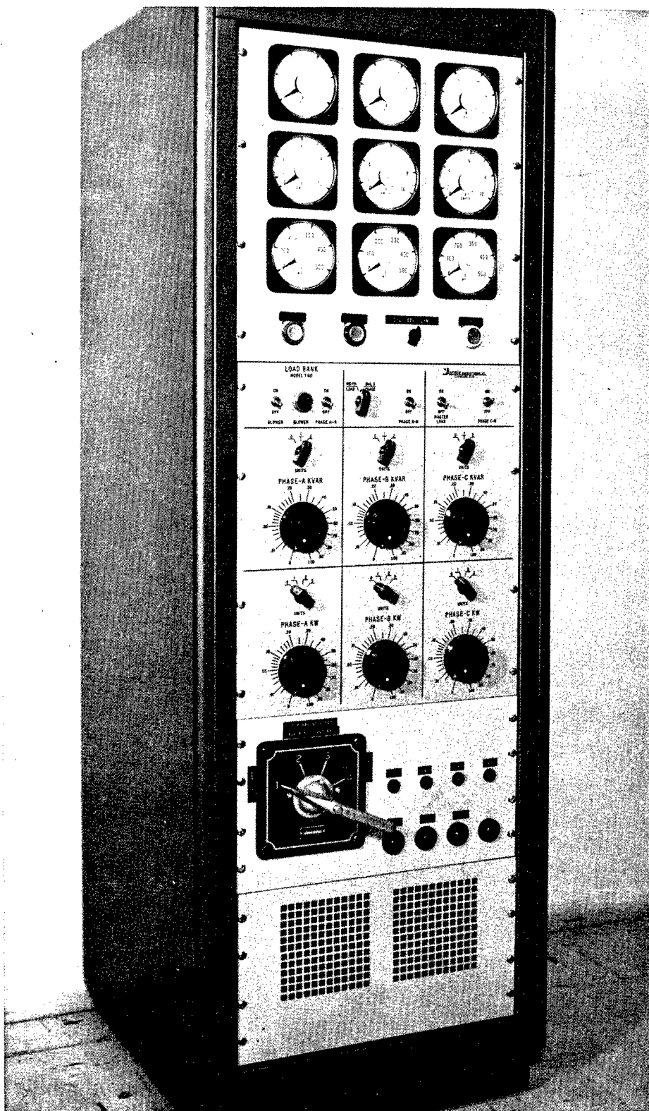
Fig. VI-11 View of the Load Bank Used to Dissipate the Power Generated During Test of the Rotor-Bearing-Alternator Simulator
