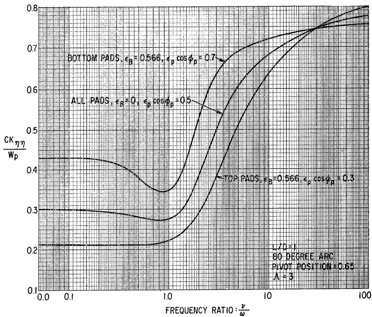
Fig. V-4 Calculated Dimensionless Pad Tangential Stiffness versus Frequency Ratio
