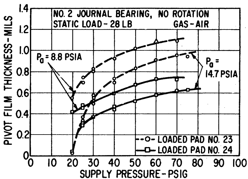
Fig. IV-7 Measured Performance of the No. 1 and No. 2 Hydrostatic Journal Bearings at 8.8 and 14.7 PSIA Ambient Pressure
