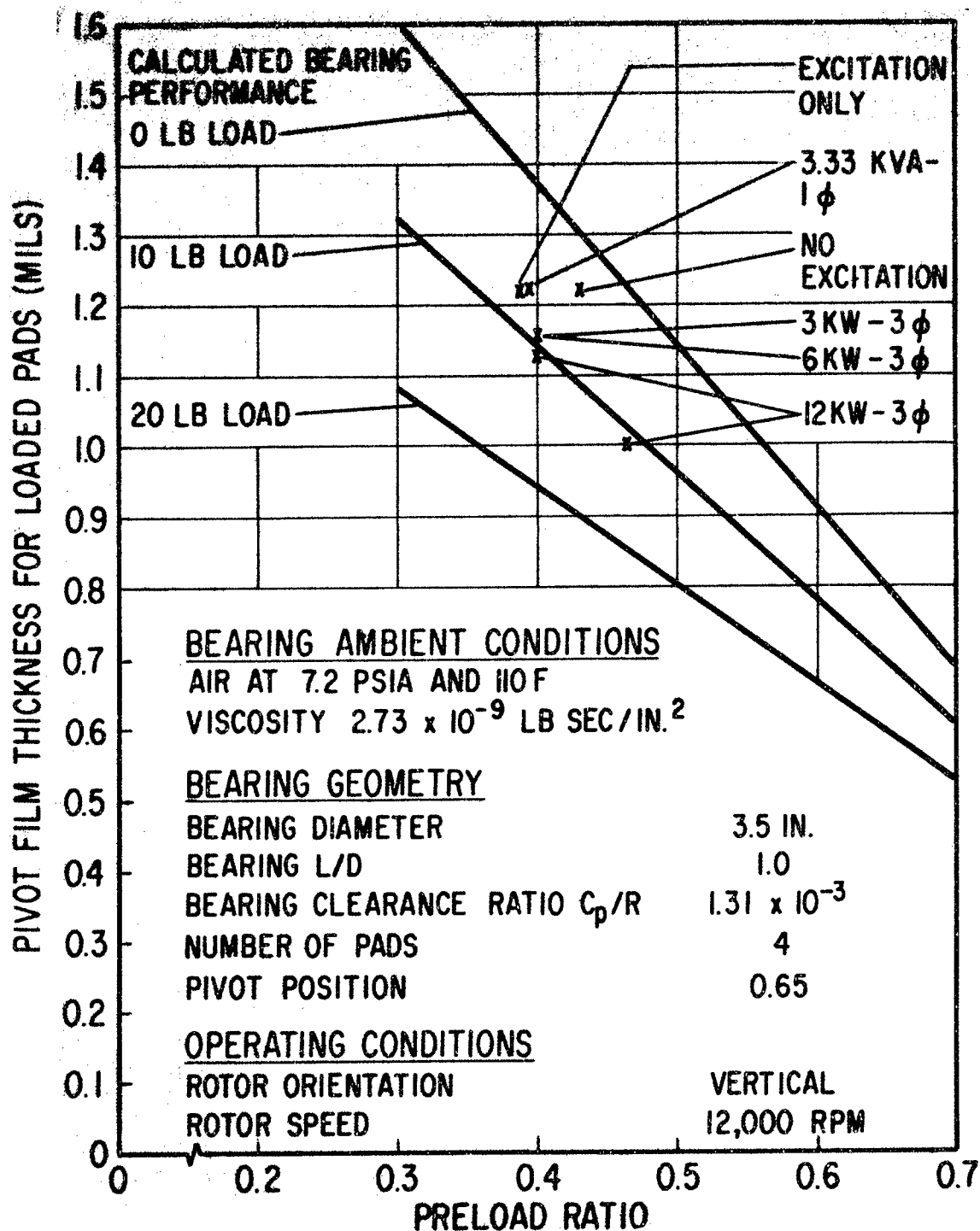
Fig. VII-18 Calculated and Experimental Performance of the Journal Bearing Adjacent to the Thrust Bearing at Low Preloads (Rotor Vertical)
