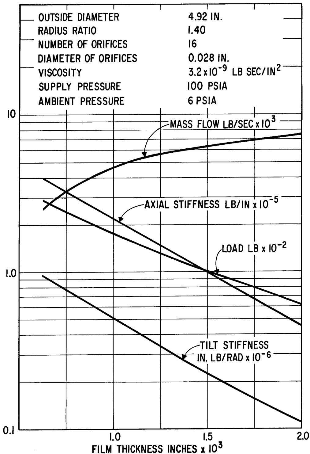
Fig. II-16 Calculated Performance of the Hydrostatic Reverse Thrust Bearing in a 6.0 PSIA Argon Environment
