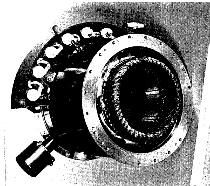
Fig. VI-8a Front View of Alternator Stator
