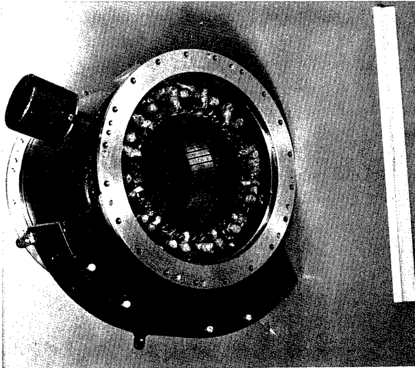
Fig. VI-8b Rear View of Alternator Stator
