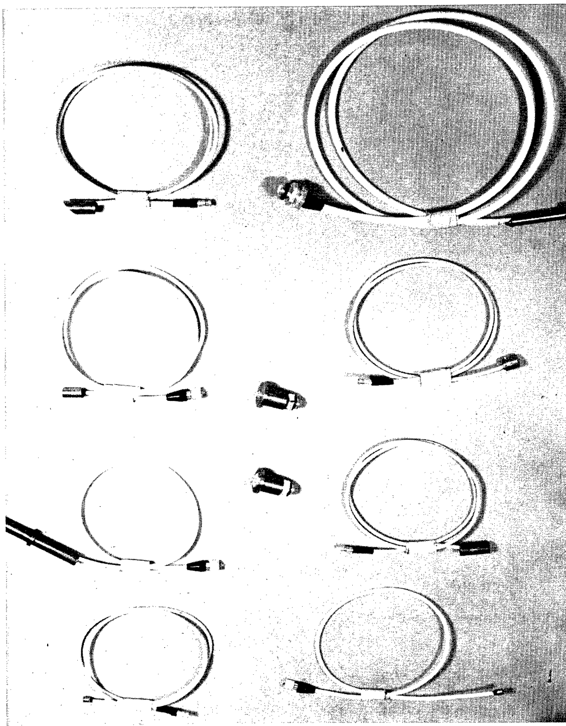
Fig. II-25 View Showing a Typical Range of Capacitance Probe Configurations for Bearing System Performance Measurement
