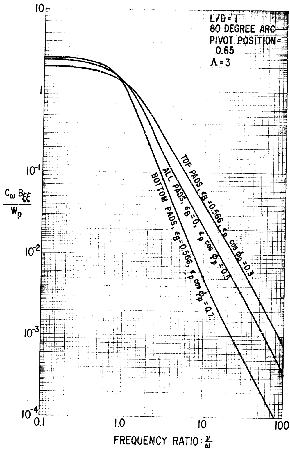
Fig. V-7 Calculated Dimensionless Pad Radial Damping versus Frequency Ratio
