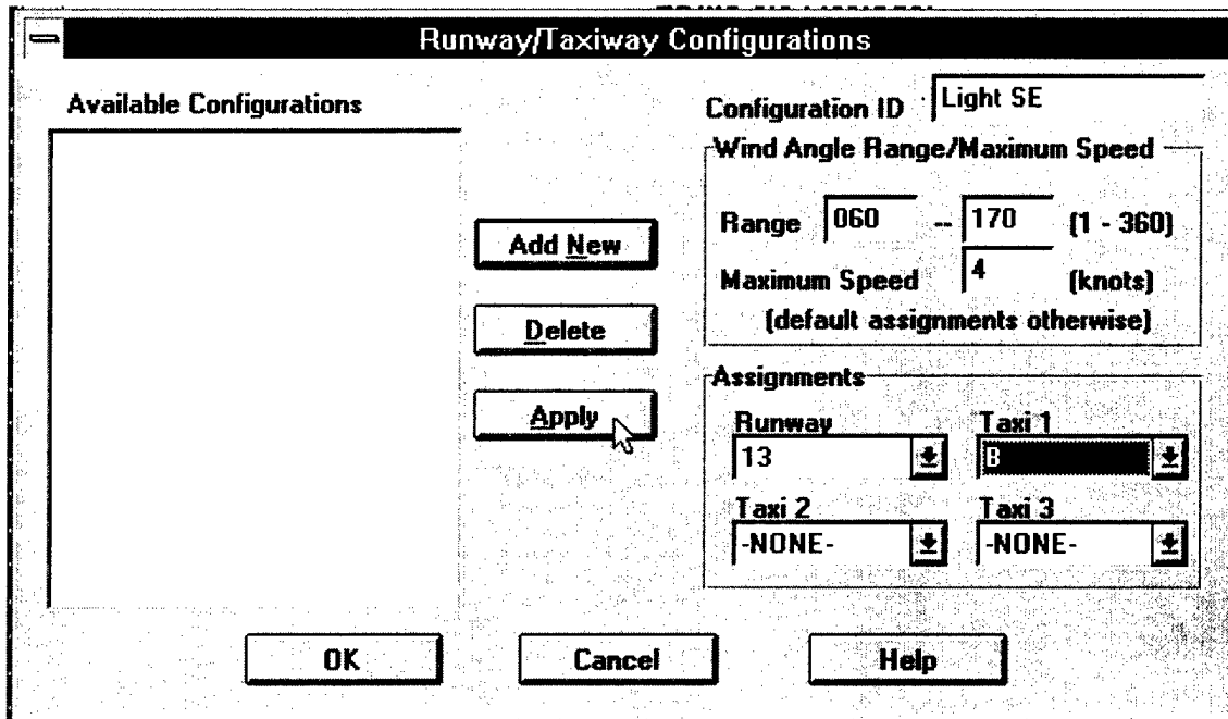
Figure 2-10: Configurations Window
