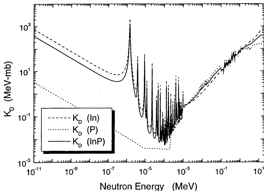
Fig. 2.7 Calculated neutron displacement kerma in In, P, and InP
