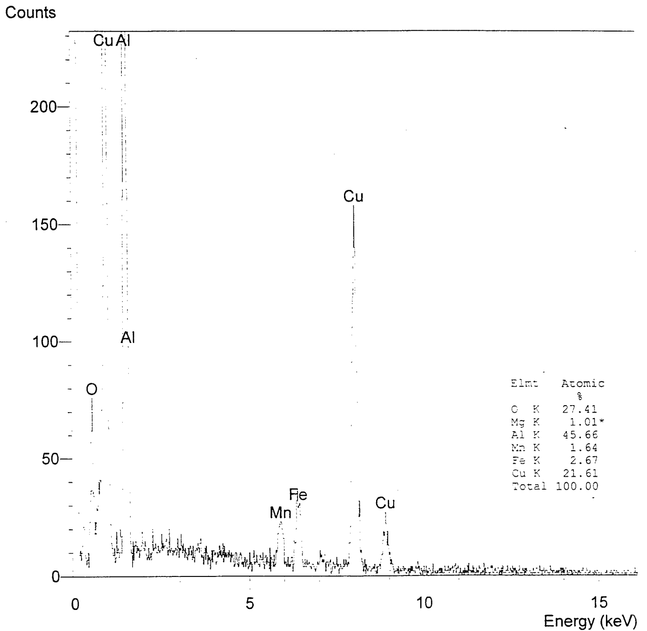
Fig.3. EDS spectrum and composition of particle on Al 2024 T3 surface (signed 1 in Fig.2) after treatment in 30 % H 3 PO 4 at 40°C for 10 min.
