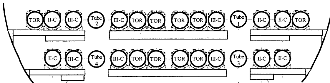
Figure 17. Forward Cutaway View of a Los Angeles Class Submarine Torpedo Room
