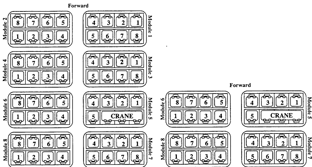
Figure 2. Full-size (left) and Half-size (right) VLS Launchers
