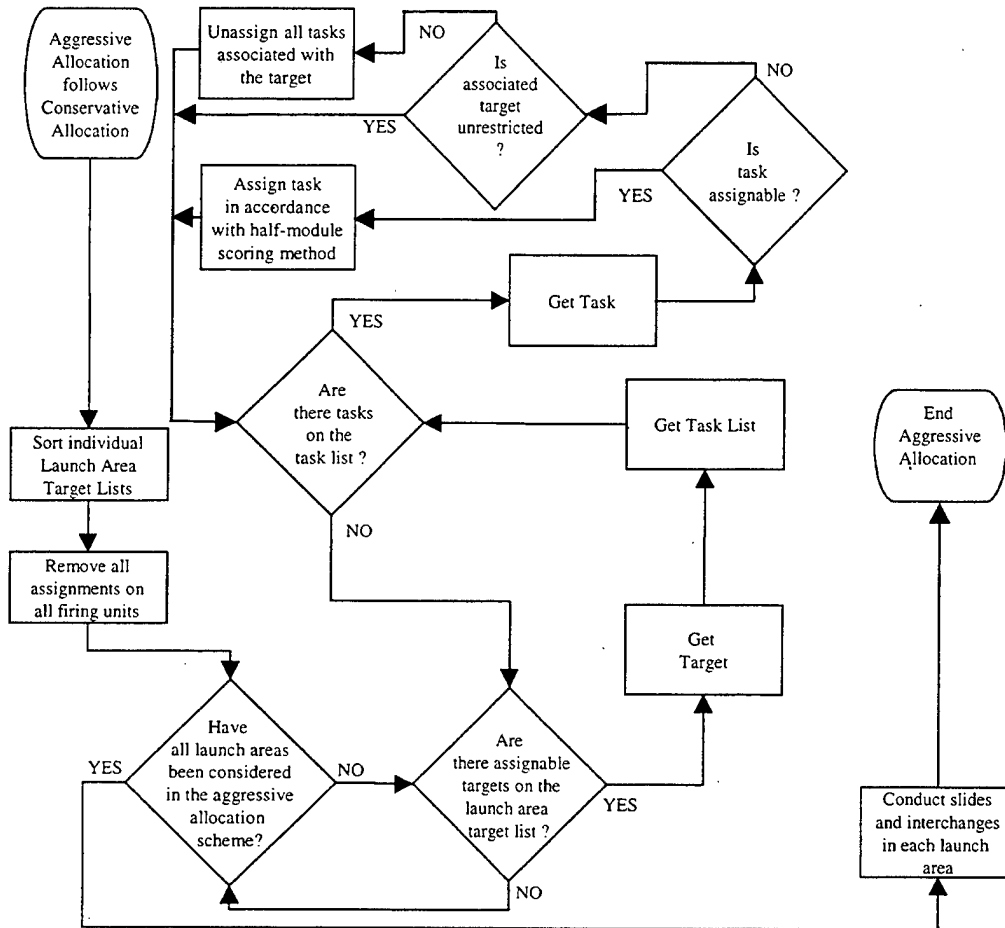
Figure 11. Aggressive Allocation
