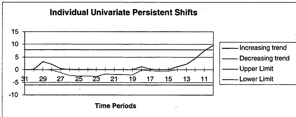
Figure 22. Individual Univariate Control Charts for Reversed SFOR Data, Threats and Rhetoric, Periods 31-10. Isolated upward departures at time periods 29 and 11. Persistent upward shift at time period 10. Persistent shift appears to begin at time period 14.
