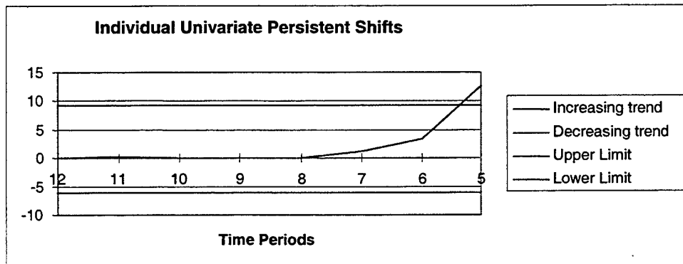
Figure 24. Individual Univariate Control Charts for Reversed SFOR Data, Threats and Rhetoric, Periods 12-5. Isolated upward departure and persistent upward shift at time period 5. The persistent upward shift appears to begin at time period 7.
