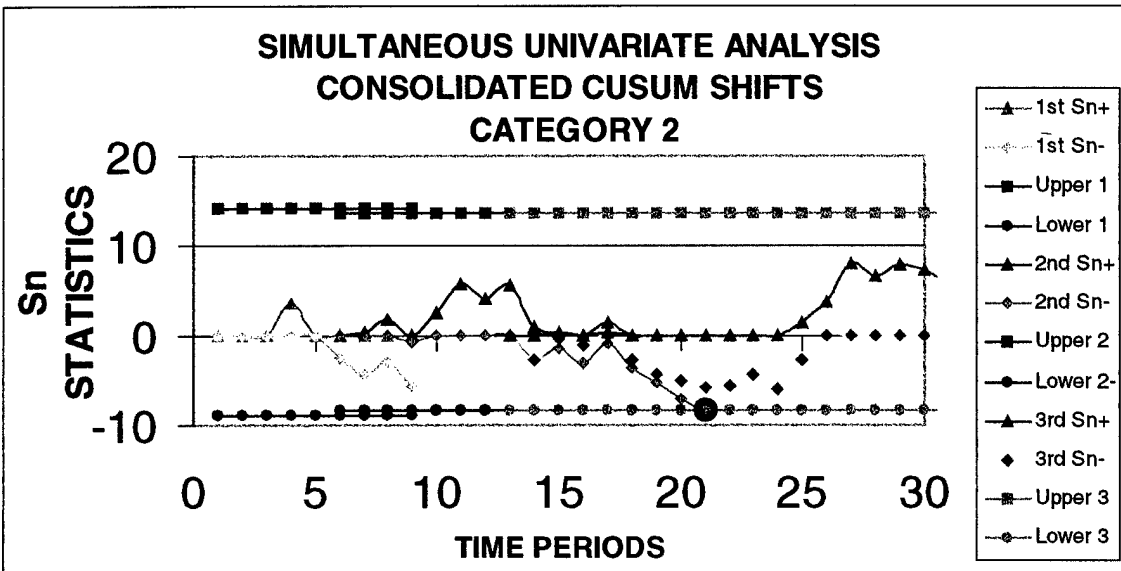
Figure 20. Simultaneous Univariate Analysis, Consolidated Shifts in Category 2. 1 st chart periods are from time period 1 to time period 9. 2 nd chart periods are from time period 6 to time period 21. 3 rd chart periods are from time period 13 to time period 31. An isolated departure occurred in time period 14. A persistent shift occurred in time period 21. Large red data point identifies shifts and departures.
