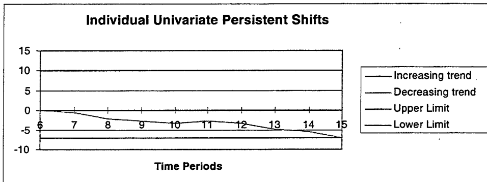
Figure 16. Individual Univariate Control Charts for SFOR Data, Threats and Rhetoric, Periods 6-15. Persistent downward shift signaled at time period 15. Decreasing trend appears to begin at time period 7.
