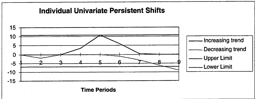
Figure 15. Individual Univariate Control Charts for SFOR Data, Threats and Rhetoric, Periods 1-9. Isolated upward departure at time period 5 and a persistent downward shift at time period 9. The persistent decreasing shift appears to begin at time period 6.
