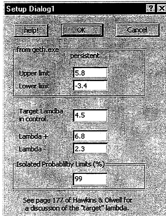
Figure 14. "Change Parameter" Dialog Box. Persistent upper and lower limits are values of the decision interval returned from ANYGETH.exe. Target Lambda in control, Lambda+, and Lambda- are parameters for which the CUSUM will be tuned to detect. The Isolated Probability Limits is the percentage used to calculate the initial Shewhart control limits.
