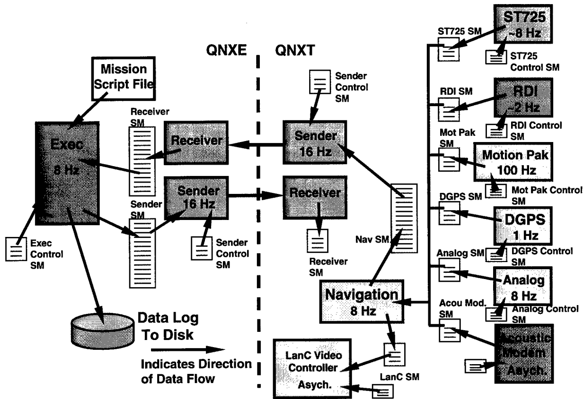
Figure 3.1: ARIES AUV Computer Architecture. [Ref. 11]
