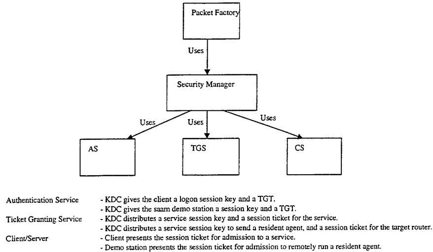
Figure 22. Security Manager Hides Kerberos Details from SAAM
