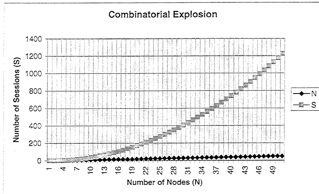
Figure 3. Combinatorial Explosion
