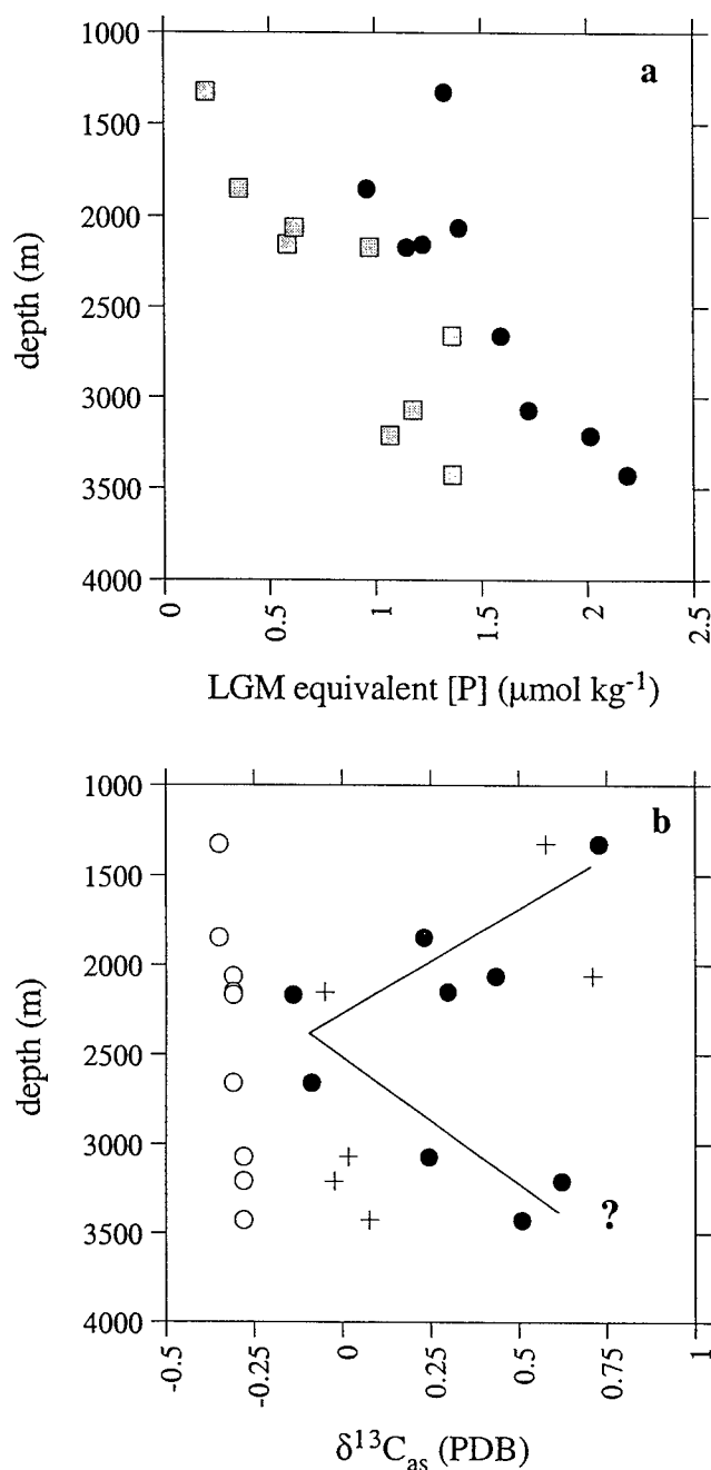
Figure 4.15. (a) LGM seawater dissolved P estimates based on published \delta^{13}\text{C} (squares) and C. wuellerstorfi Cd/Ca from this study (circles). (b) \delta^{13}\text{C}_{\text{as}} estimates based on modern water column data (open circles; Lynch-Stieglitz and Fairbanks, 1994) and on the LGM data in panel (a) (filled circles). Lines represent a possible LGM relationship, but it is questionable whether or not the deepest \delta^{13}\text{C}_{\text{as}} estimates are accurate. Note that the Holocene foraminifera from these cores (crosses) do not give a good match to the modern water column data, mainly because of Cd/Ca values that are higher than expected.
