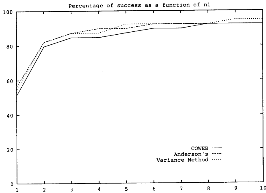
Figure 42: Influence of n_1 values over percentage of success.
