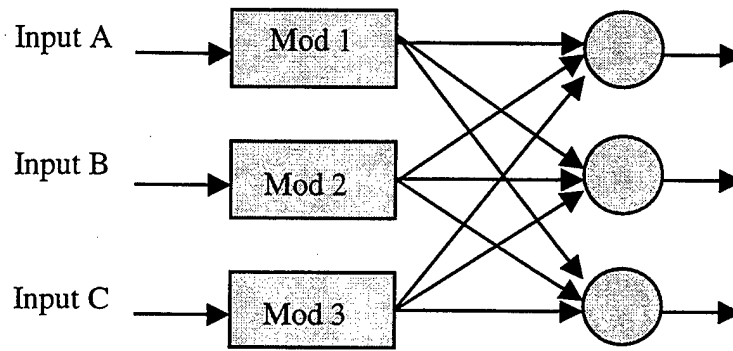
Figure 2.3. Triplicated TMR Voters. After Ref. [7]
