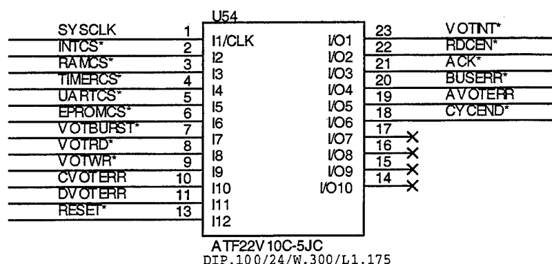
Figure 4.2. Memory Controller PLD
