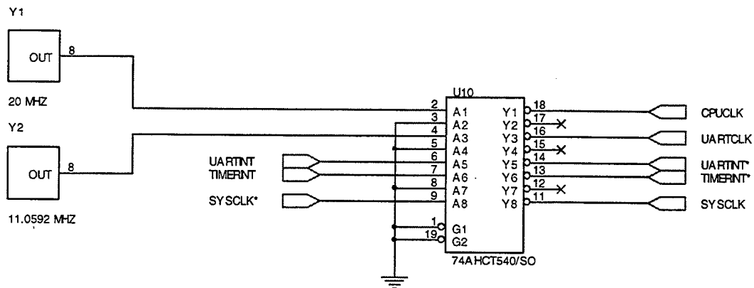
Figure 3.2. Timing Interface
