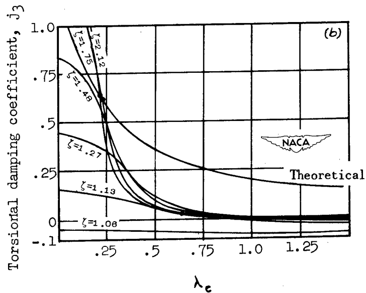
Figure 65.- Effect of torsional damping coefficient j_3 on flutter for different frequency ratios ( \zeta = \omega_\alpha / \omega_b ). Reference 3.
