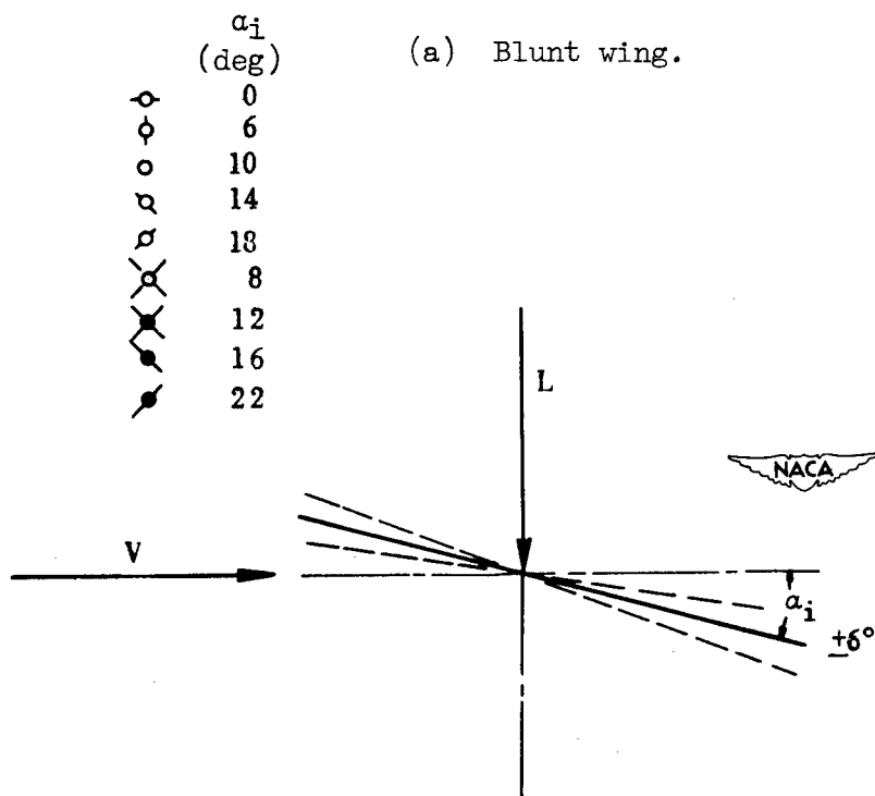
Figure 18.- Lift amplitude in pure pitch.
