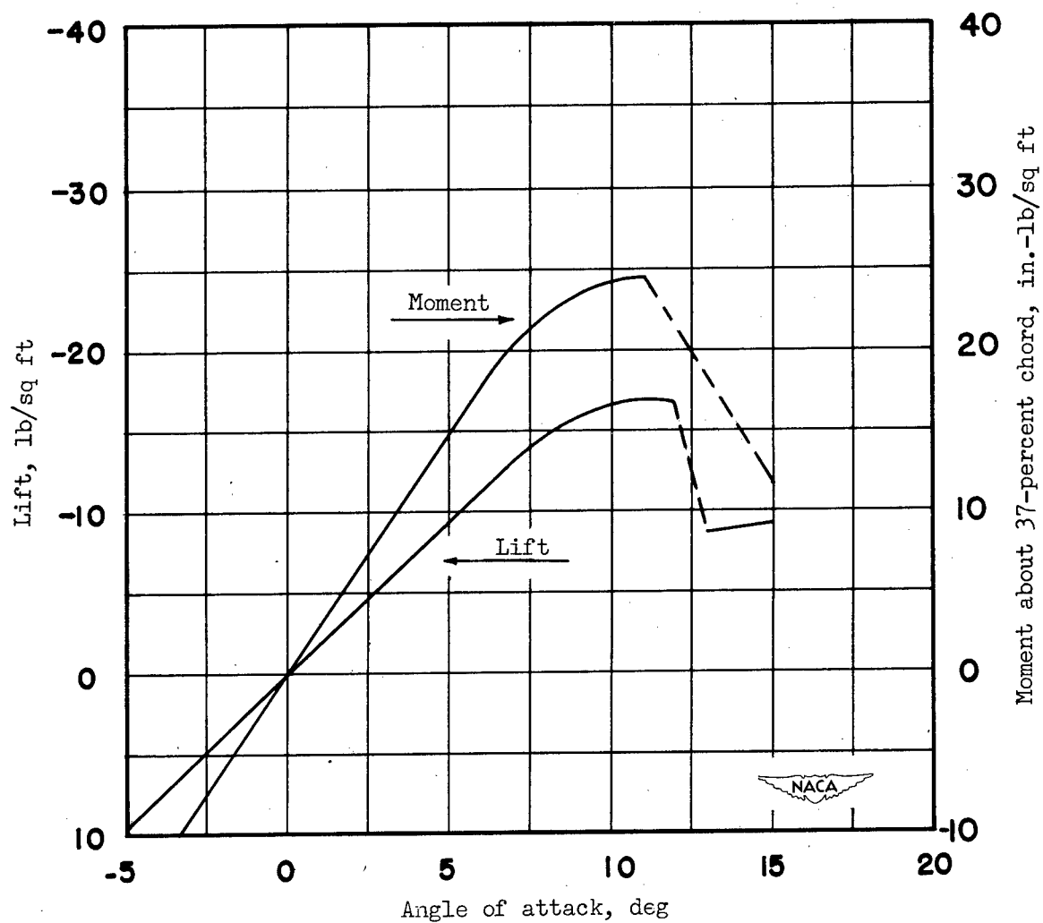
Figure 9.- Static airfoil characteristics. Sharp airfoil.
