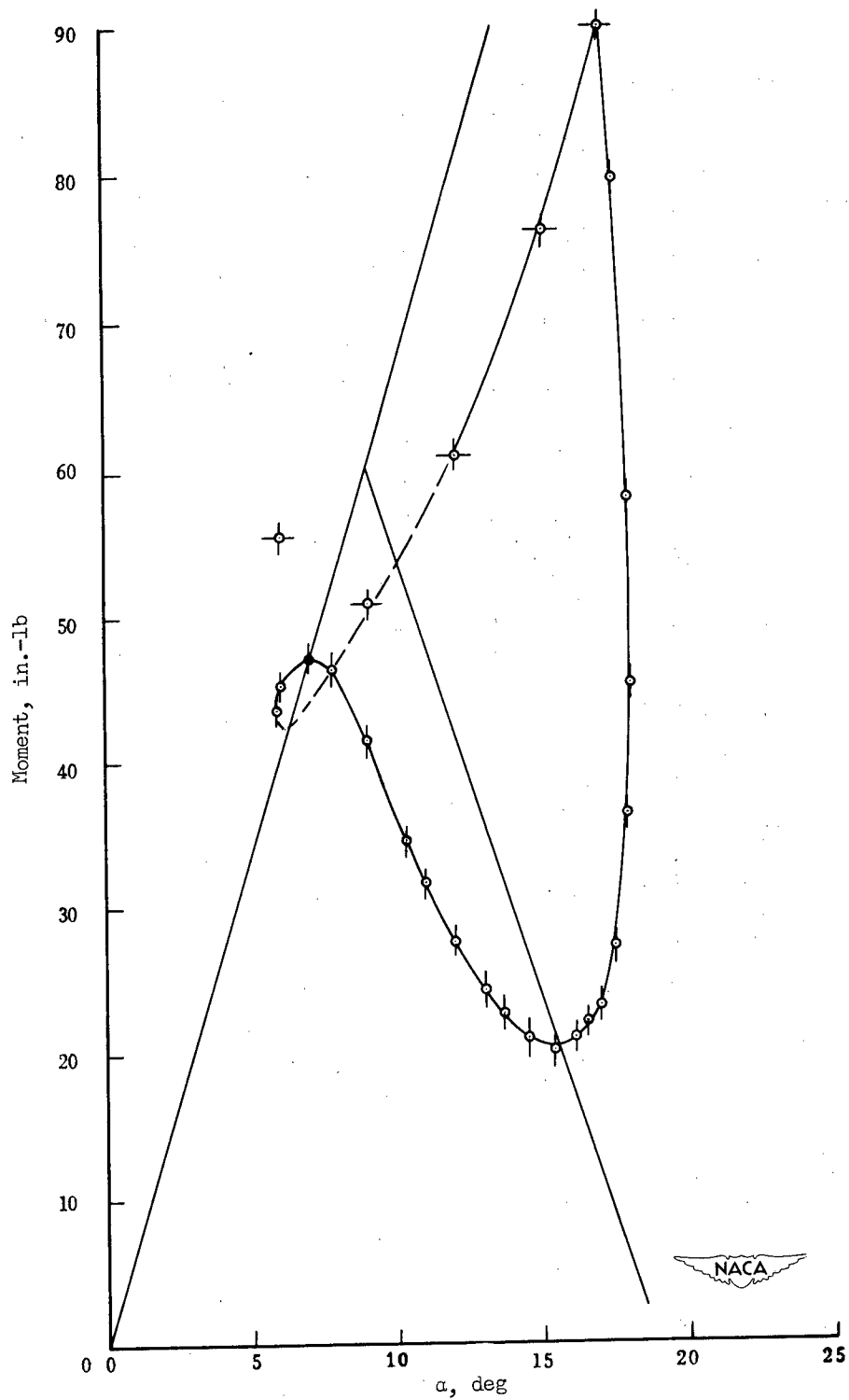
Figure 71.- Hysteresis loops from empirical theory. Sharp airfoil.
