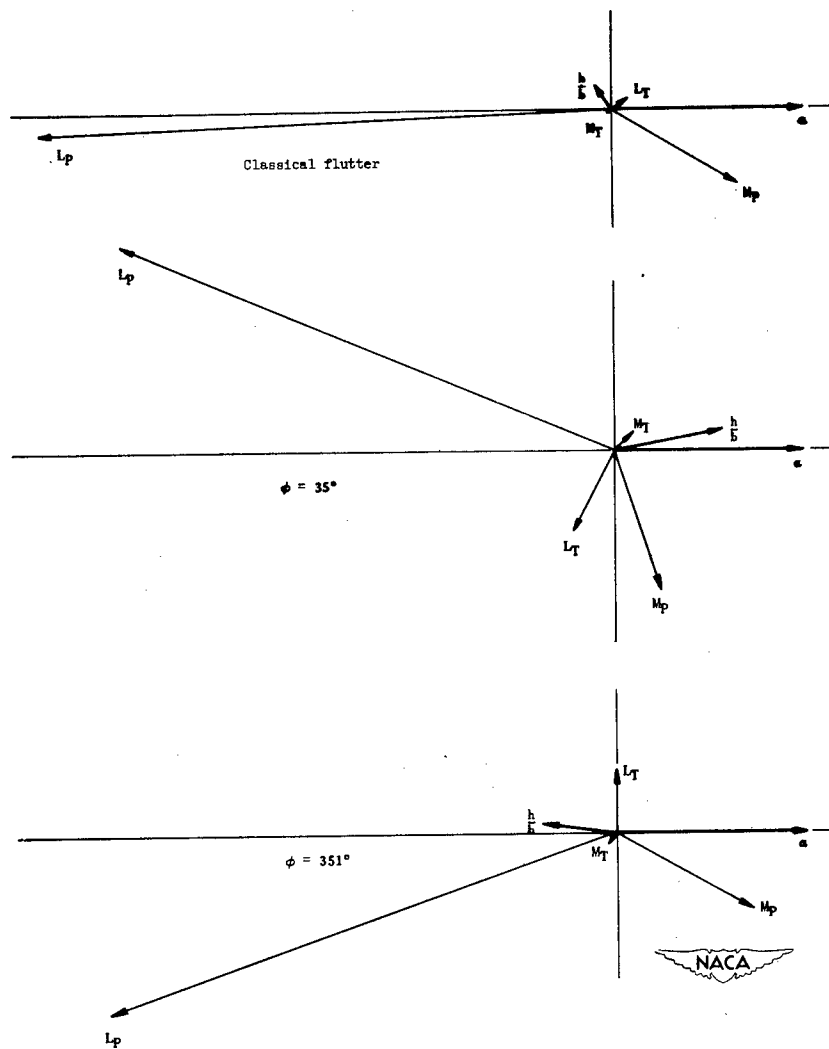
Figure 67.- Vector plots of aerodynamic derivatives at flutter.
