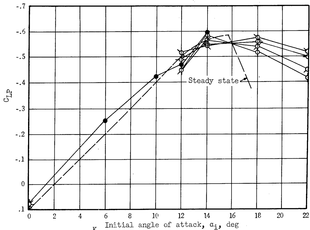
(a) Blunt wing.
