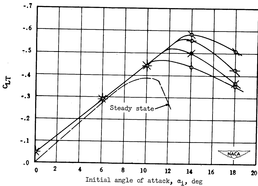
(c) Sharp wing.
