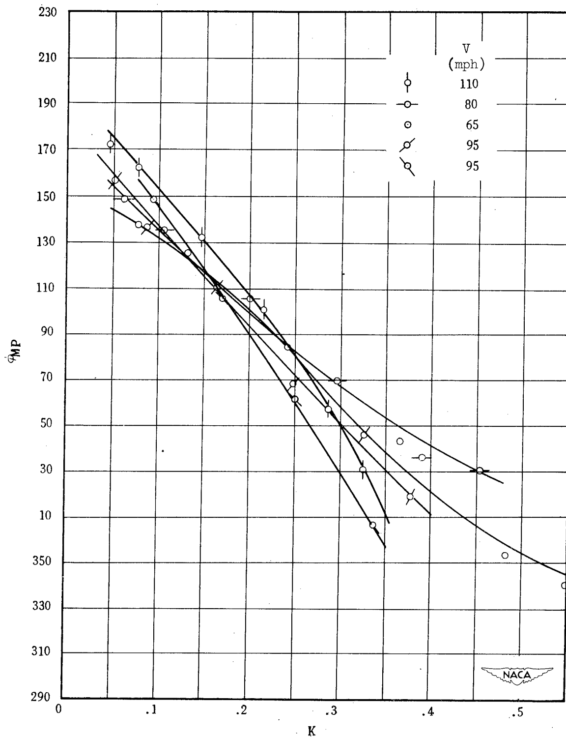
Figure 31.- Moment phase angle in pure pitch from harmonic analysis. Intermediate wing. \alpha_i = 14^\circ ; \Delta\alpha = 0^\circ .
