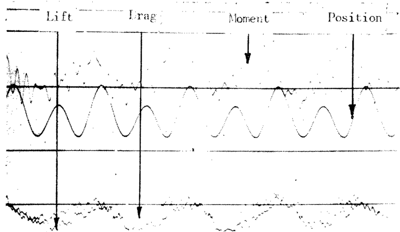
(c) \alpha = 14^\circ ; \omega = 7.58 cycles per second. Lift attenuation, 1-5; moment attenuation, 1-3; drag attenuation, 1-2.
