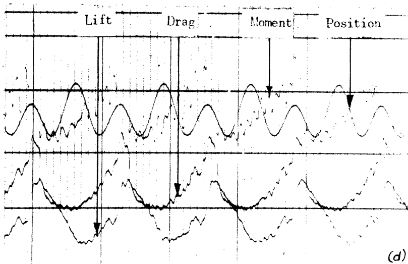
(d) \alpha = 18^\circ ; \omega = 8.2 cycles per second. Lift attenuation, 1-10; moment attenuation, 10-1; drag attenuation, 1-10.
