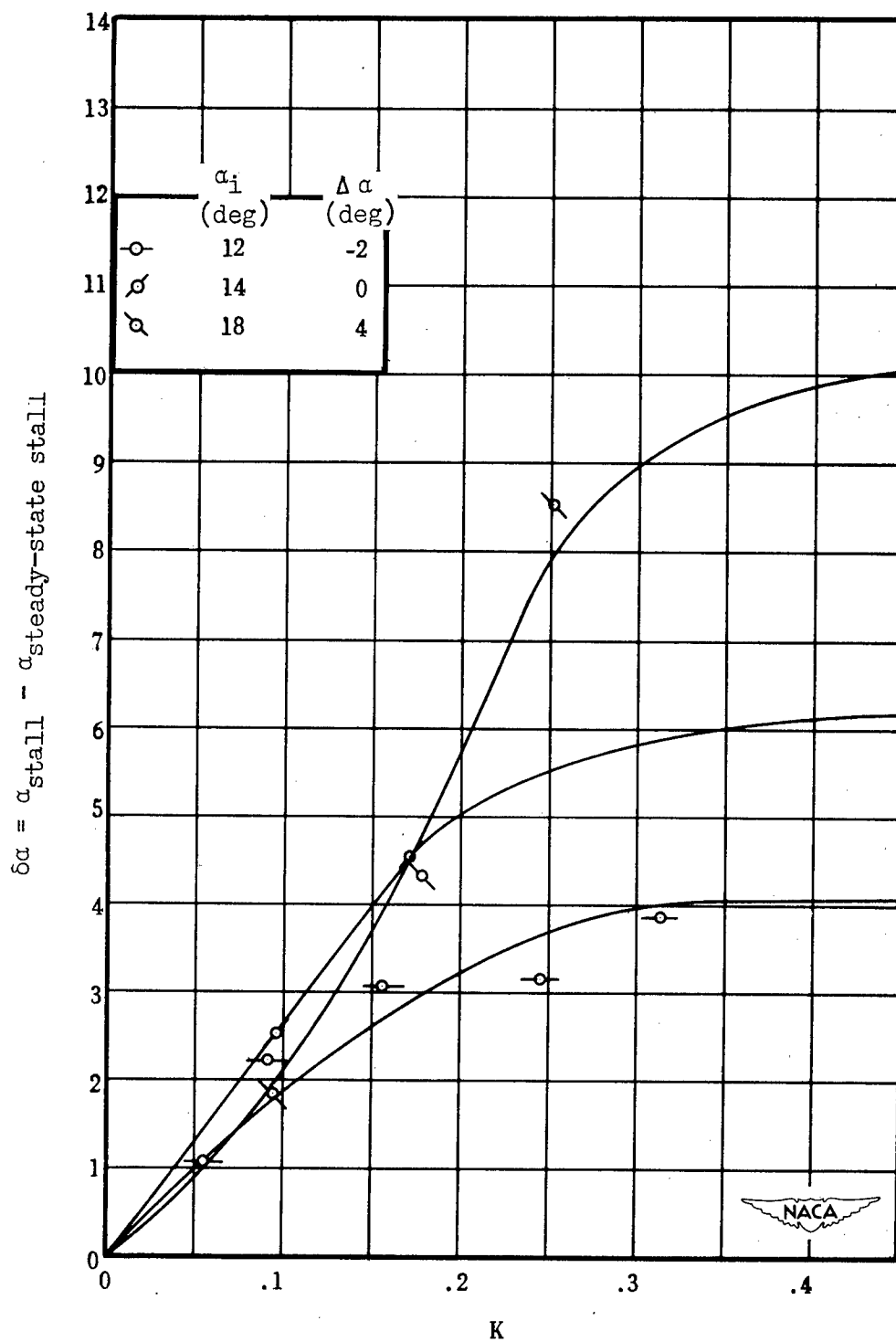
Figure 43.- Oscillatory stalling angle as a function of K . Intermediate wing.
