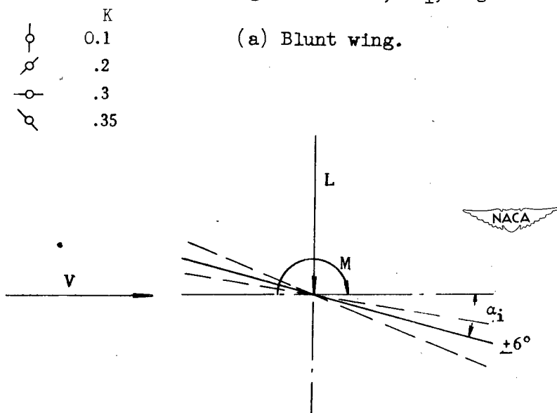
Figure 33.- Time-average value of moment in pure pitch.
