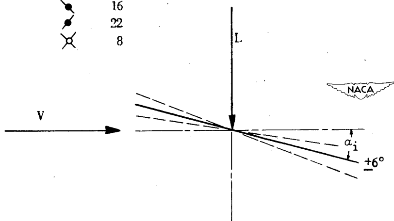
Figure 14.- Lift phase angle in pure pitch.
