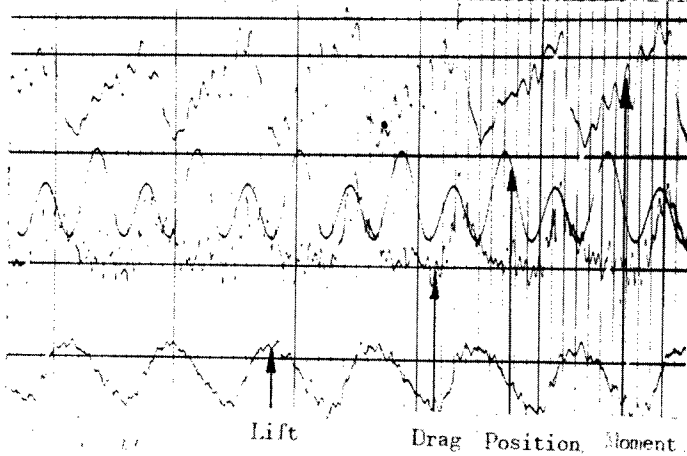
Figure 54.- Effect of frequency of oscillation. Sharp wing. Pure translation.
