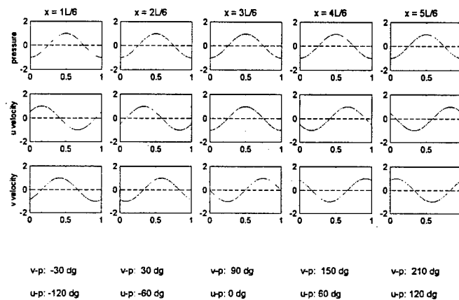
Figure 4.19: Idealized description of phase between velocity components and cavity pressure as a discrete vortex convects along the cavity opening at a constant speed
