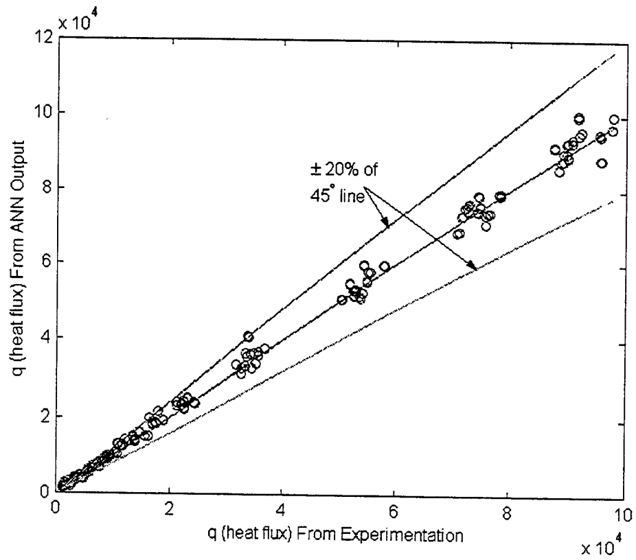
Figure 22: Plot of the Output of the ANN vs. the Experimentation for Different Numbers of Active Tubes.
