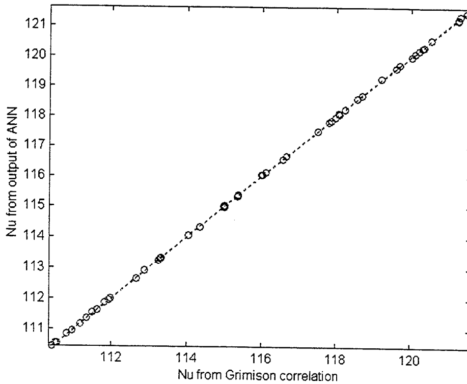
Figure 12: Plot of Neural Network Output (ANN) vs. the Values Attained by the Grimison Correlation. This is a Portion of the Previous Figure Shown in More Detail.
