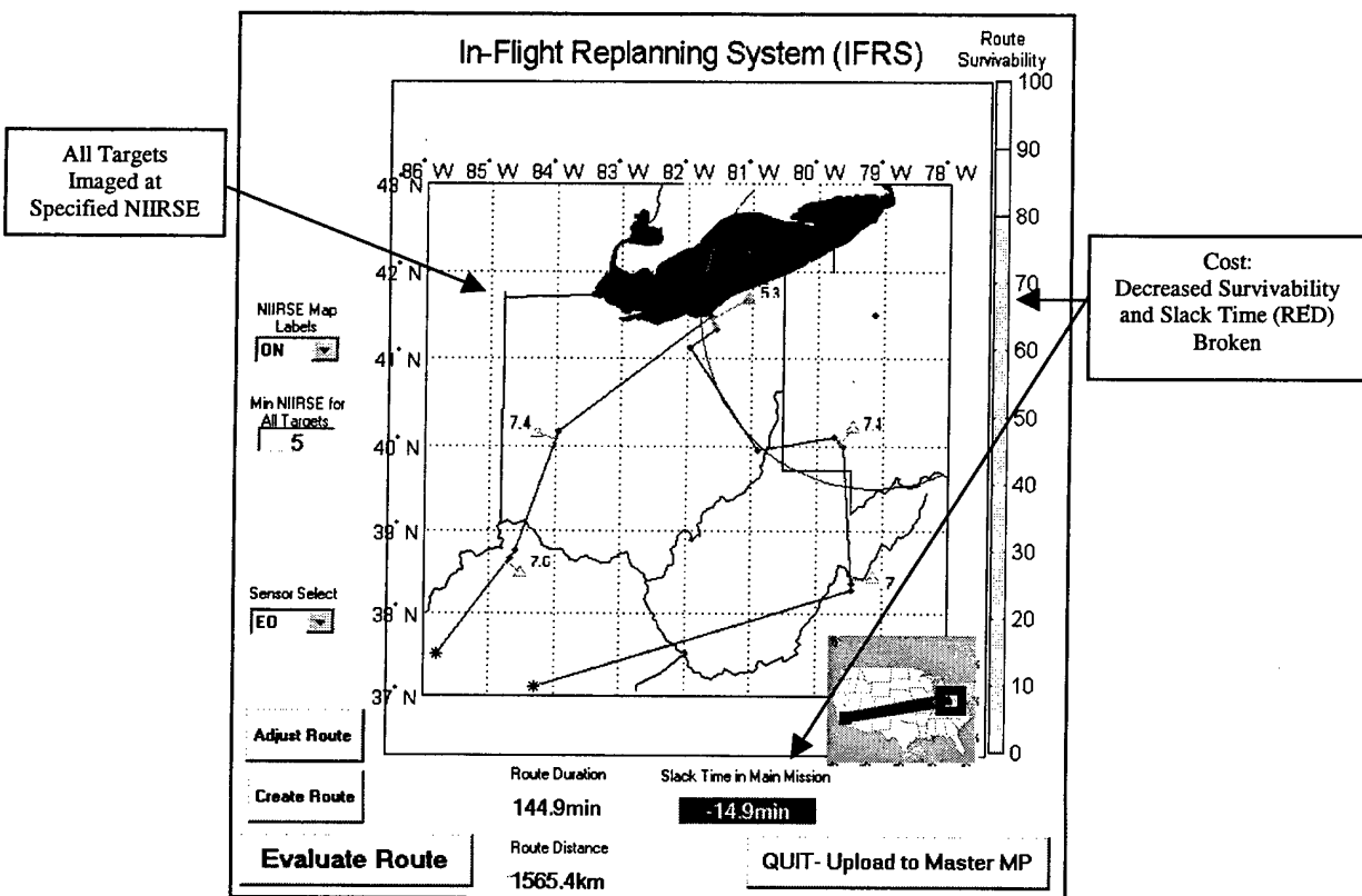
Figure 17 Replan Option 1: Break TOT Constraint
