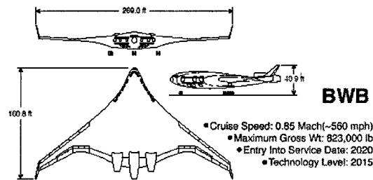
Figure 2-4: BWB 3 View
