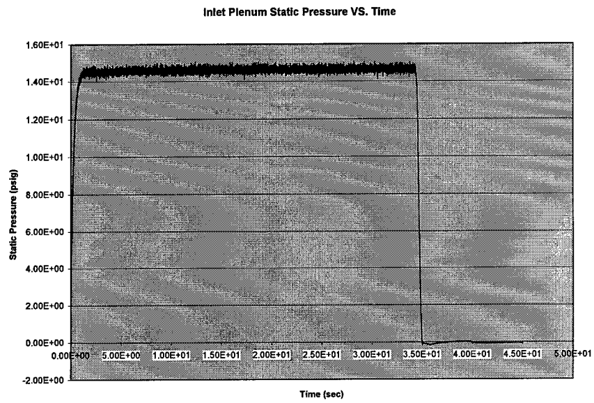
Figure 20. Inlet Plenum Static Pressure
