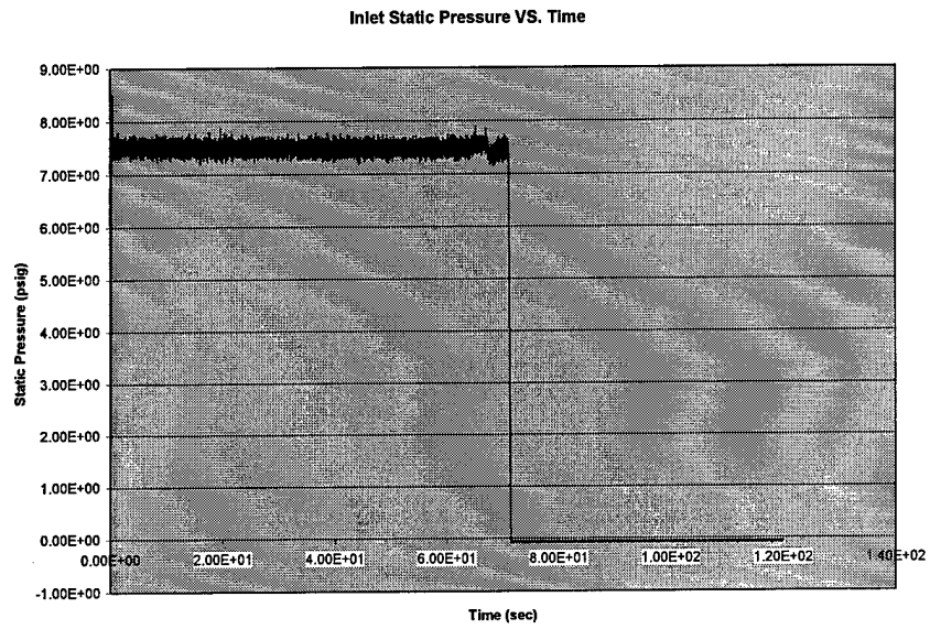
Figure 15. Inlet Plenum Static Pressure
