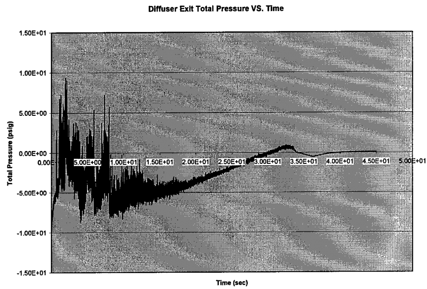
Figure 33. BL1 Diffuser Exit Total Pressure
