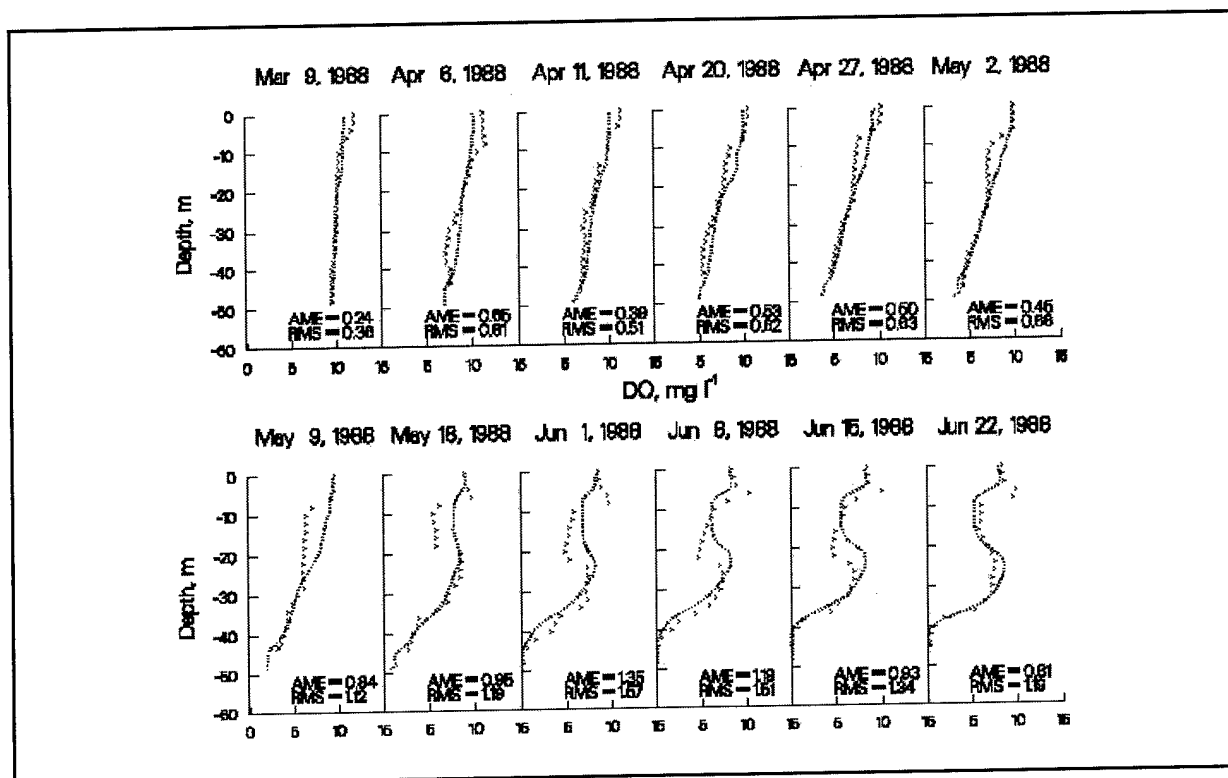
Figure 10. 1988 RBR computed versus observed DO, March-June
