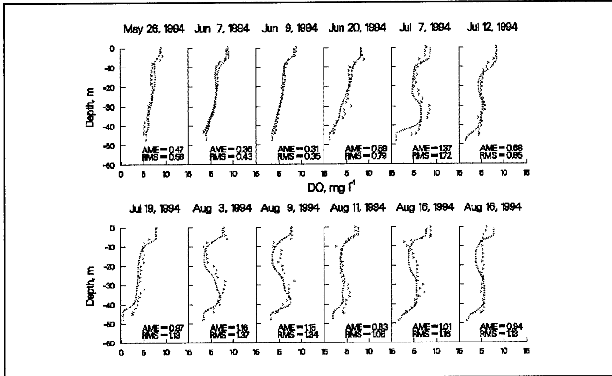
Figure 12. RBR 1994 computed versus observed DO
