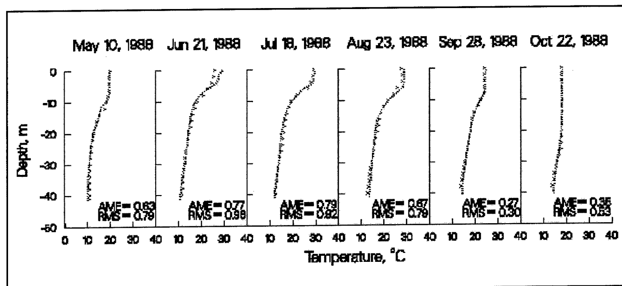
Figure 7. 1988 JST computed versus observed temperature
