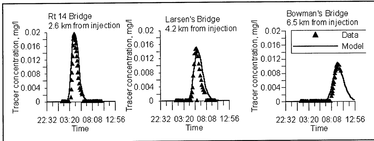
Figure 25. June 1999 Lower Bull Run River computed versus observed dye concentrations
