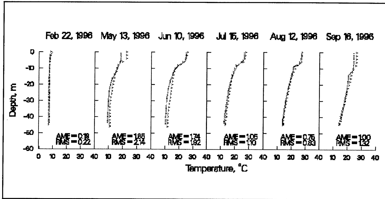
Figure 9. 1996 JST computed versus observed temperature
