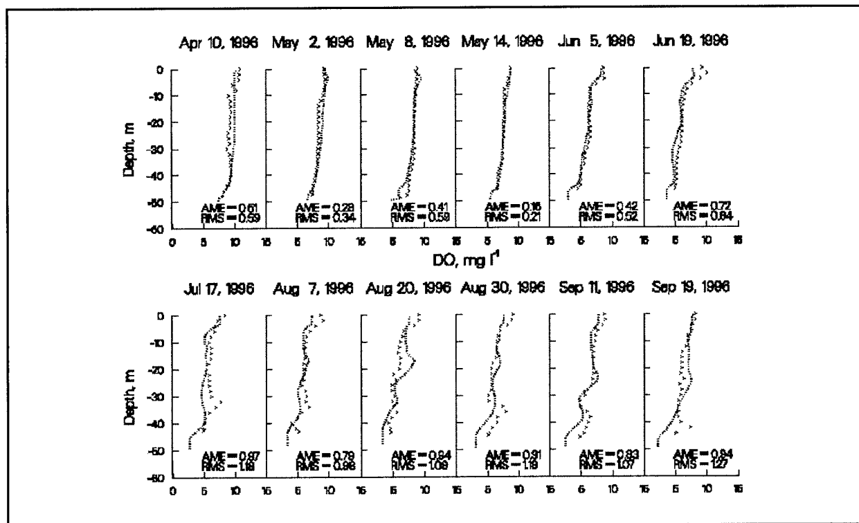
Figure 13. 1996 RBR computed versus observed DO
