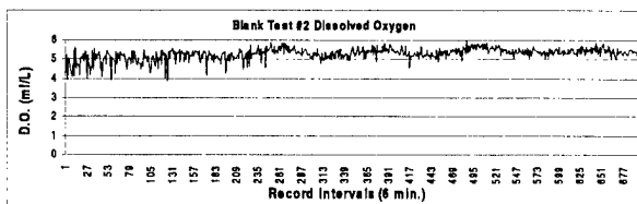
Figure 30. Blank test for dissolved oxygen
