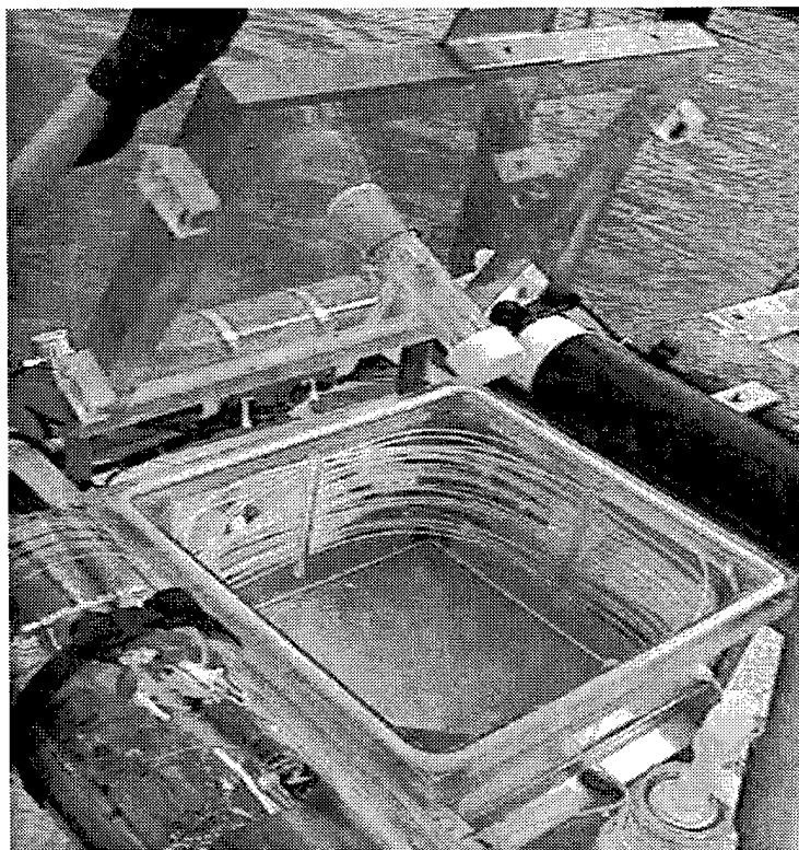
Figure 7. Chamber enclosure.
