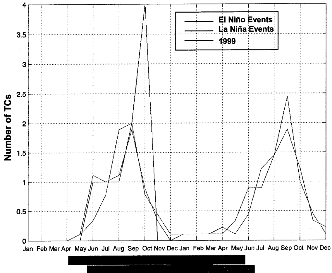
Figure 38. The average number of weak ( <80 knot ( 41 \text{ ms}^{-1} ) maximum intensity) Atlantic TCs per month for composite El Niño and La Niña events, based on nine strong events and for 1999. Red and blue bars at bottom of figure indicate the duration of composite El Niño and La Niña events, with event peaks indicated in darker colors. The TC season in this region extends from April to December. This study focuses on the first season shown in this figure, the season that occurs during and immediately before the event peaks (see Chapter 2 for rationale). See Chapter 2 for information on evolution of events and selection of event years.
