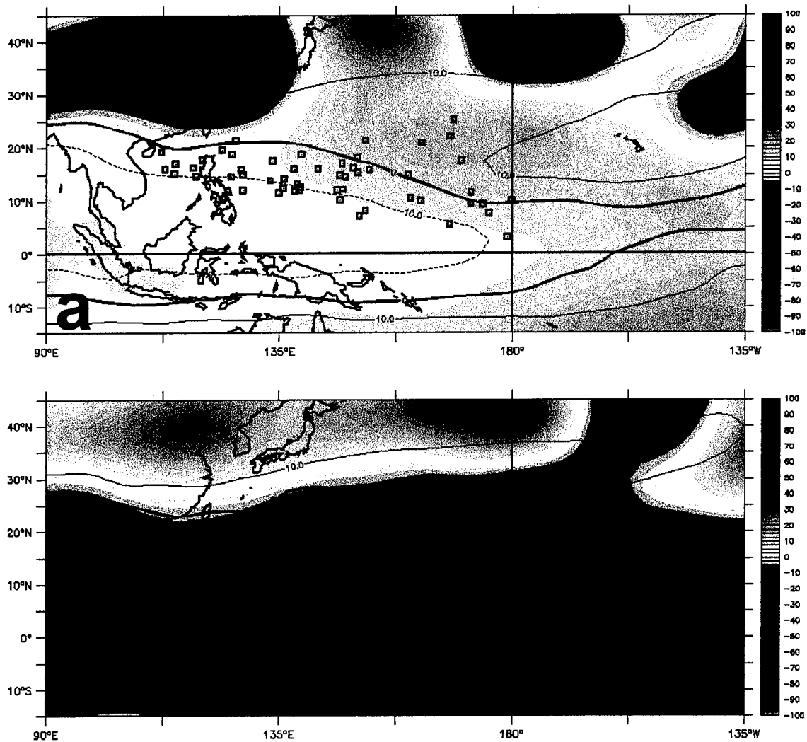
Figure 16. September tropical cyclone formation sites with composite 200 hPa anomalous geopotential heights (filled color in m) and actual shear (contour lines in ms -1 ) based on nine strong events for: (a) El Niño and (b) La Niña .
