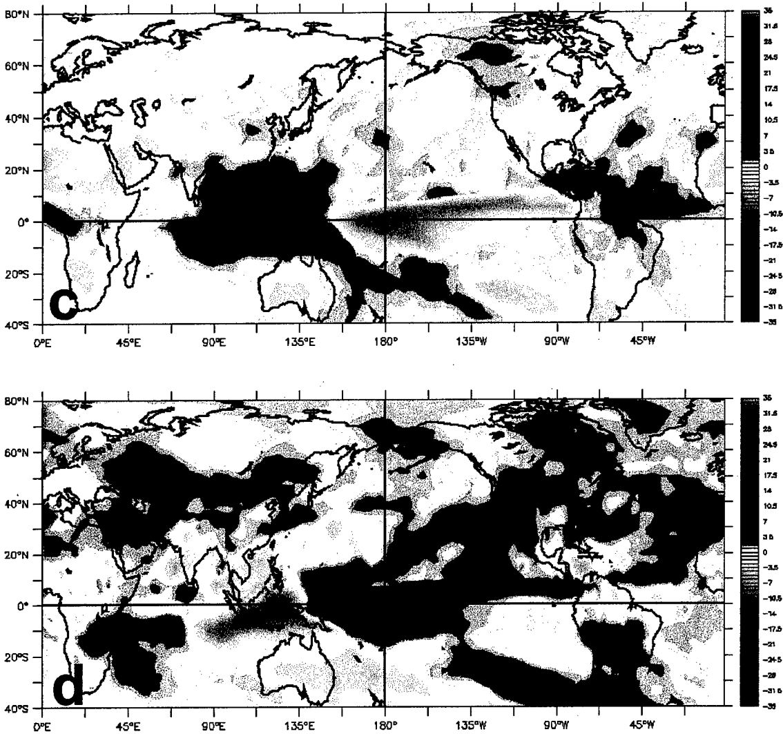
Figure 33 (continued). Composite anomalies for August-November prior to El Niño or La Niña event peak: (c) El Niño OLR anomalies in Wm^{-2} ; (d) La Niña OLR anomalies in Wm^{-2} . See Chapter 2 for information on evolution of events and selection of event years.
