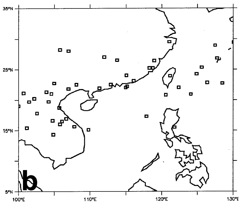
Figure 30. September tropical cyclone points of westernmost longitude for nine strong events . Red squares indicate El Niño storms and blue indicates La Niña storms for (a) the western Pacific and (b) the South China Sea.
