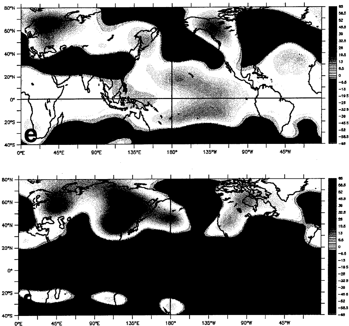
Figure 33 (continued). Composite anomalies for August-November prior to El Niño or La Niña event peak: (e) El Niño 200hPa geopotential ( Z_{200} ) height anomalies in m; (f) La Niña 200hPa geopotential height anomalies ( Z_{200} ) in m. See Chapter 2 for information on evolution of events and selection of event years.
