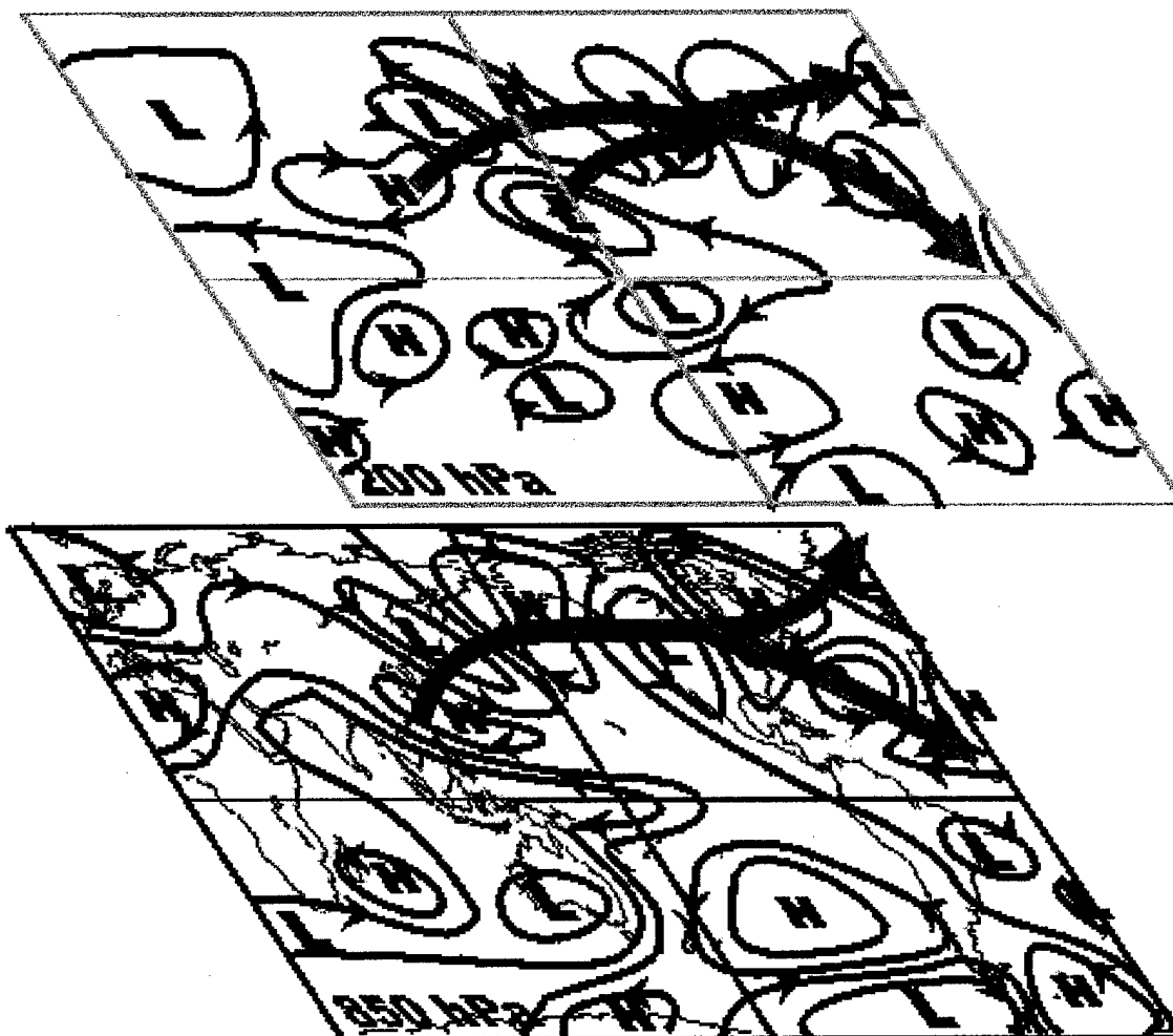
Figure 47. Schematic representation of anomalous circulation brought about by La Niña events during August-November to the event peak.
