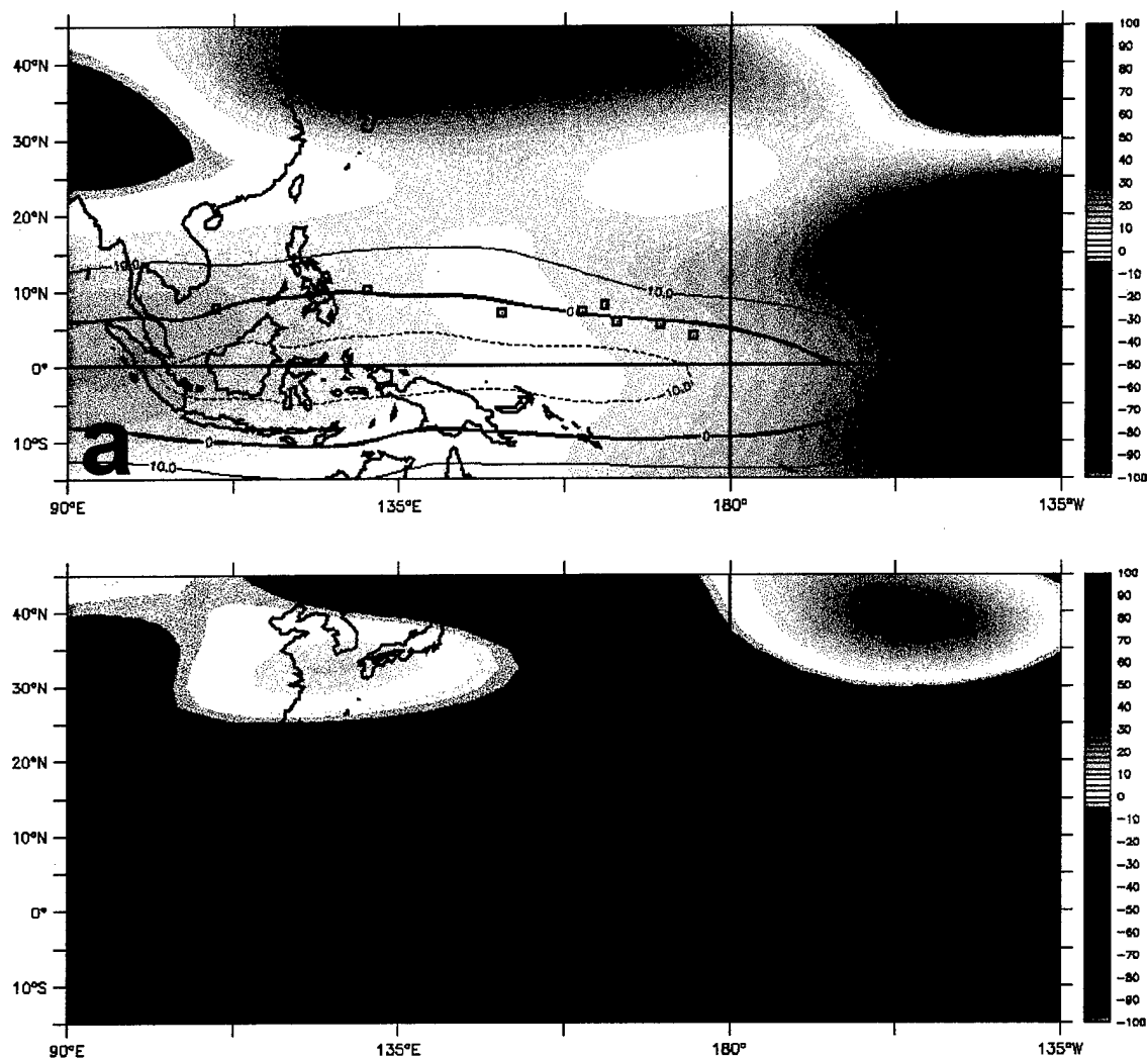
Figure 19. December tropical cyclone formation sites with composite 200 hPa anomalous geopotential heights (filled color in m) and actual shear (contour lines in \text{ms}^{-1} ) based on nine strong events for: (a) El Niño and (b) La Niña .
