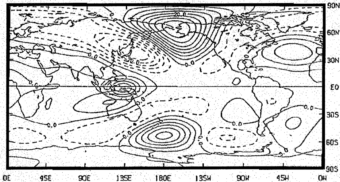
Figure 2. Modeled geopotential height response at 200 hPa to a positive tropical heating perturbation centered on the equator at 130E (indicated by oval contours). Positive (negative) height responses are indicated by solid (dashed) contours. Height contour interval = 5 m. The background flow is zonally symmetric with 25 \text{ ms}^{-1} jets at 25^\circ\text{N} and 32^\circ\text{S} . The arching pattern of positive and negative height responses over the East Asian – North Pacific – North American – North Atlantic region reveals a quasi-stationary wave train initiated by the perturbation heating. A similar wave train occurs over the Australian – South Pacific – South Atlantic region.
