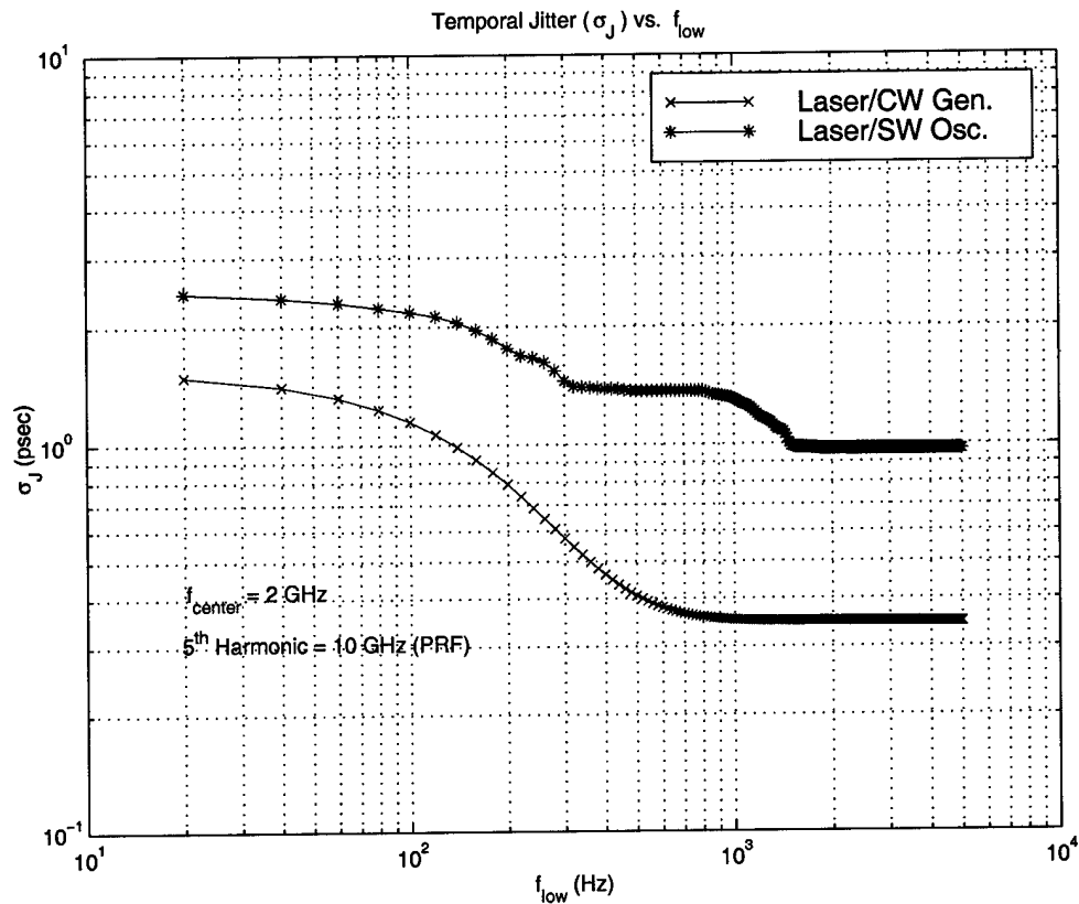
Figure 4.14. Laser powered by CW generator and sweep oscillator, timing jitter comparison.
