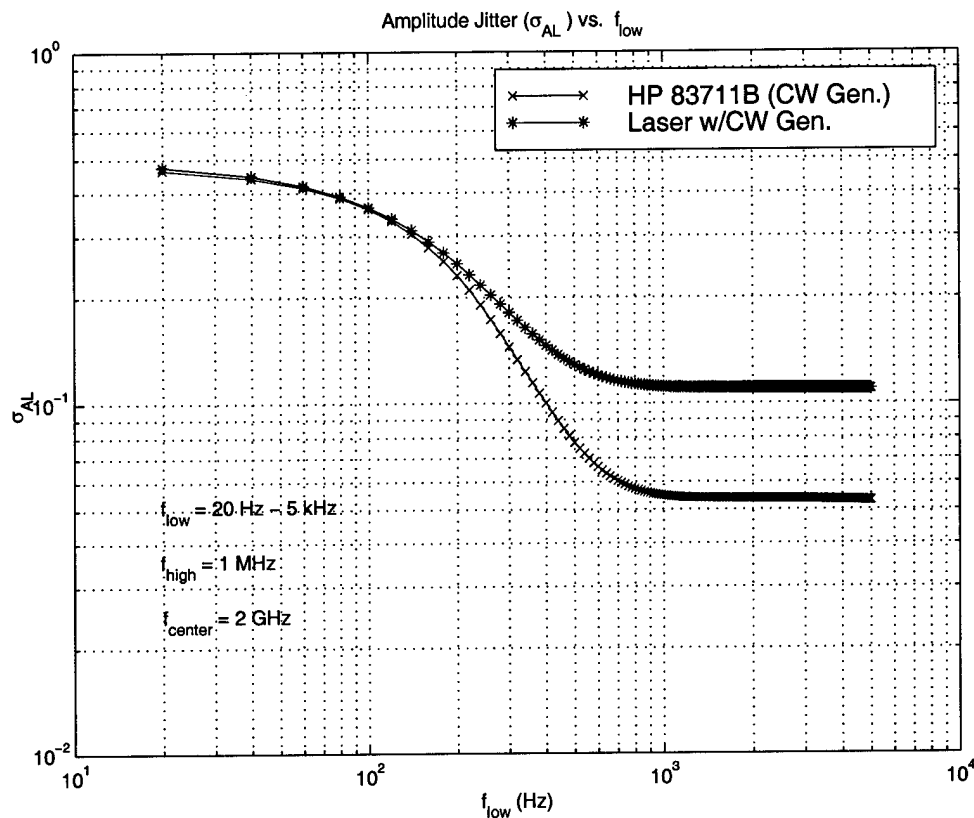
Figure 4.11. CW generator and laser powered by CW generator, amplitude jitter comparison.
