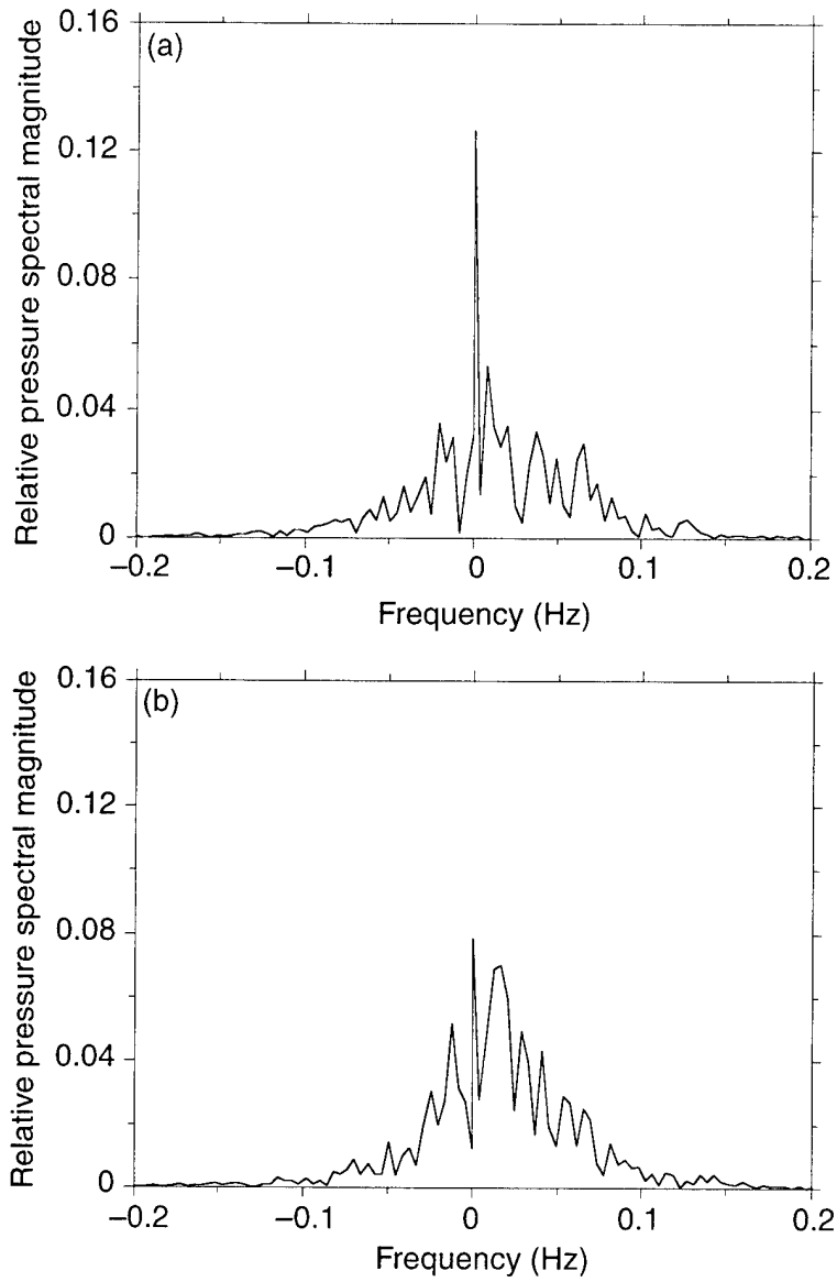
Figure 14. Signal frequency spectrum scattered by temperature fluctuations for one tube of 1.5-m turbules, randomly spaced, (a) all with \Gamma_T > 0 and (b) with \pm\Gamma_T equally likely.
