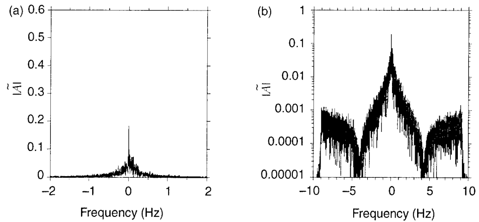
Figure 16. (a) Total frequency spectrum due to temperature and velocity fluctuations for two full tubes located above the two tubes in figure 14, with sizes 1.5 m down to 4.7 cm. (b) Log plot of (a) from \pm 10 Hz.
