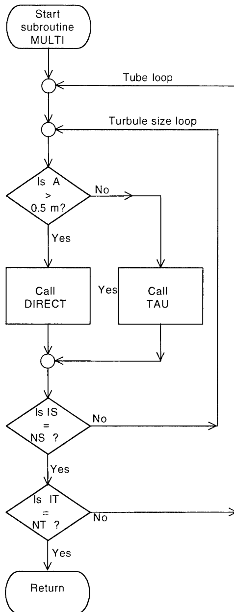
Figure D-3. Flow chart for subroutine MULTI.
