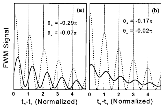
Fig. 4 Calculated time-integrated FWM response for the upper (solid lines) and lower (dashed lines) cavity-polariton modes. Nonlinear processes including band filling, local field, and EID are included. The time delay is normalized to the oscillation period. (a) \delta=0 . (b) \delta=1 .
