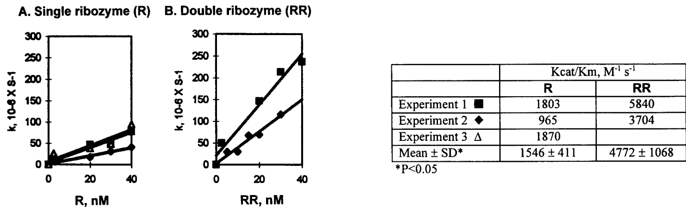
FIG. 4. Comparison of single and double RZs in vitro by single-turnover experiments. Single turnover experiments with RZ in excess over substrate were carried out and K cat /K m values were calculated as described in Materials and Methods . In Exps 1 and 2, R and RR were assayed in parallel.
