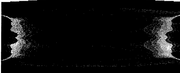
Figure 15: Minimum-Volume RADICL intensity contours ( W/m^2 ).
