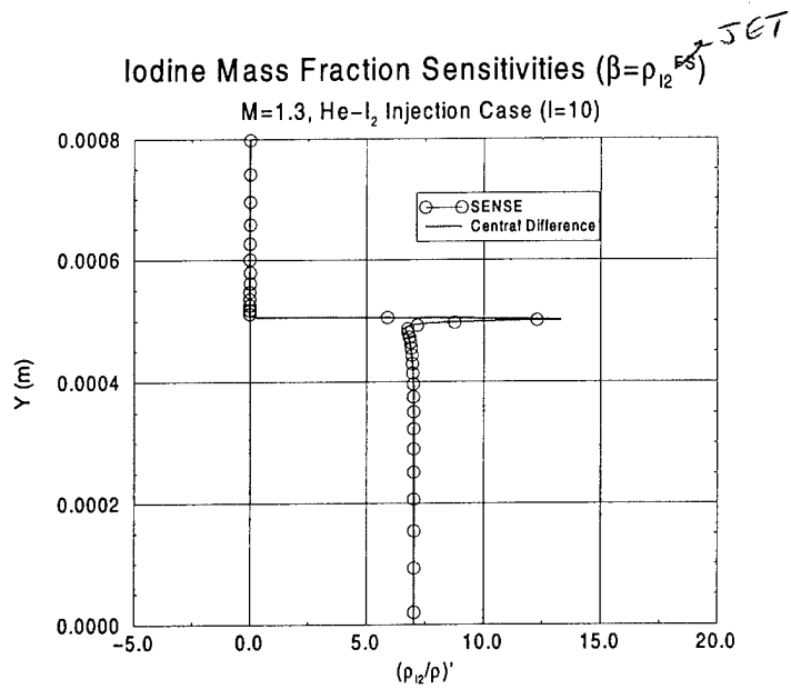
(a) Iodine mass fraction sensitivities (station I=10).
