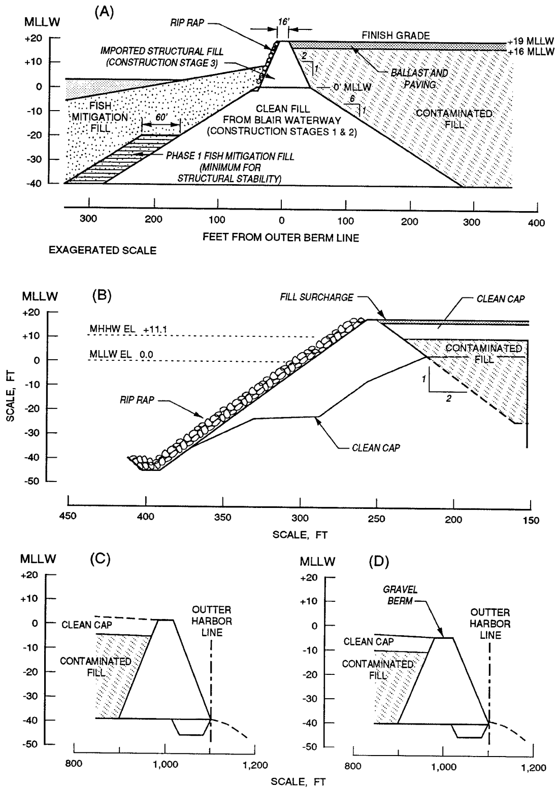
Figure 16. Cross section of the dike for the nearshore CDF conceptual design (To convert feet to meters, multiply by 0.3048)
