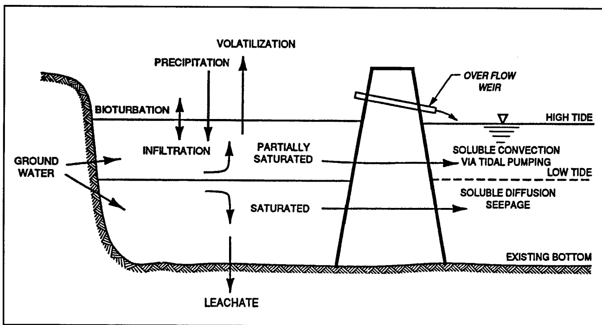
Figure 13. General contaminant pathways for nearshore CDFs
