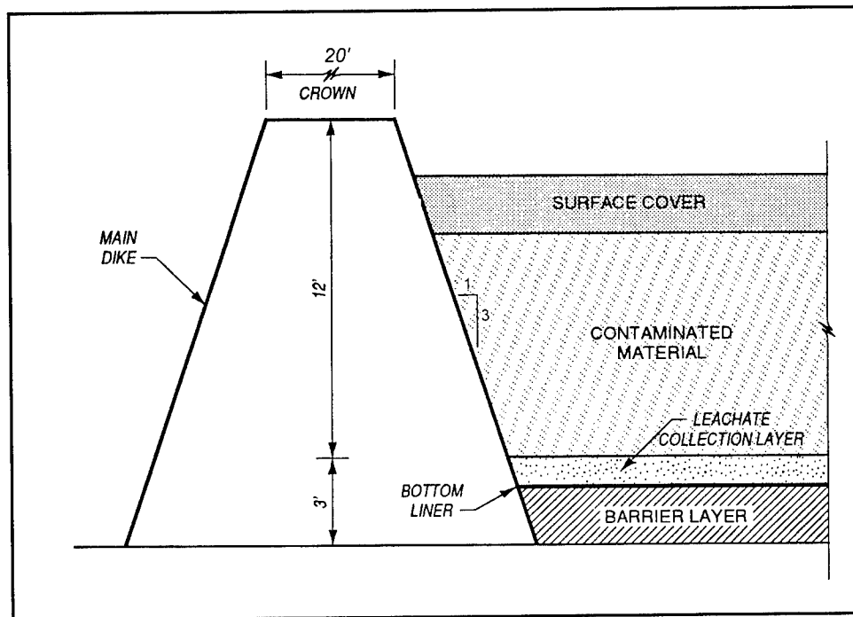
Figure 11. Cross section of the lined cell for upland CDF conceptual design (To convert feet to meters, multiply by 0.3048)
