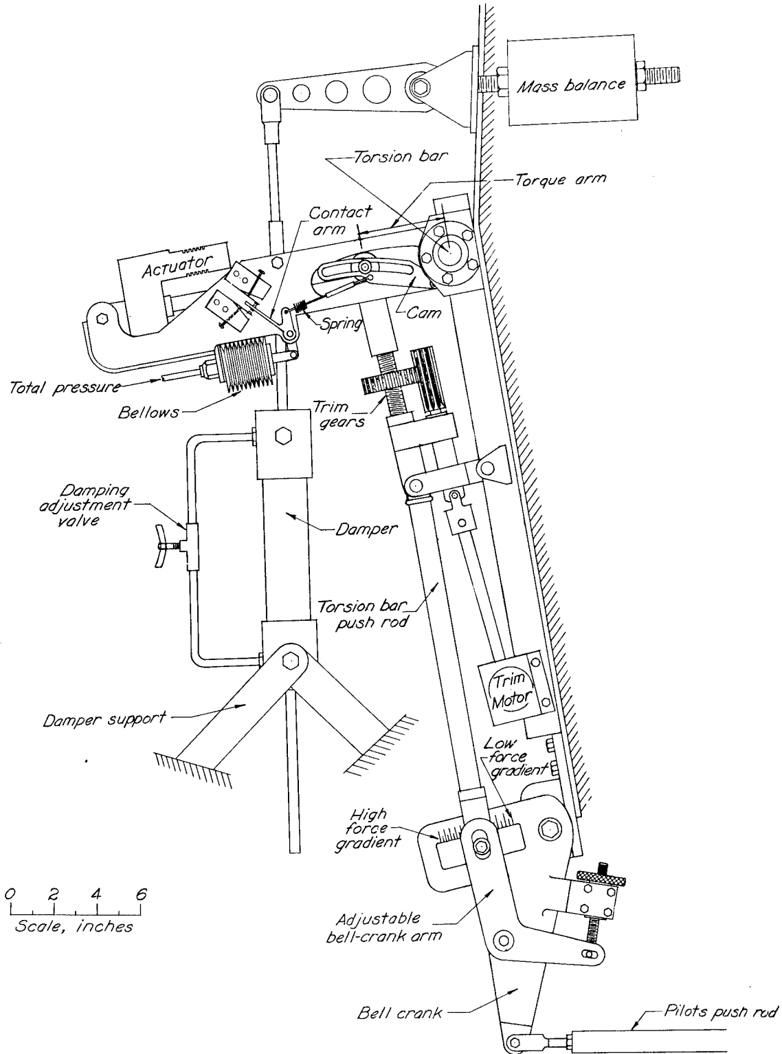
Figure 4.- Scale drawing of feel device.
