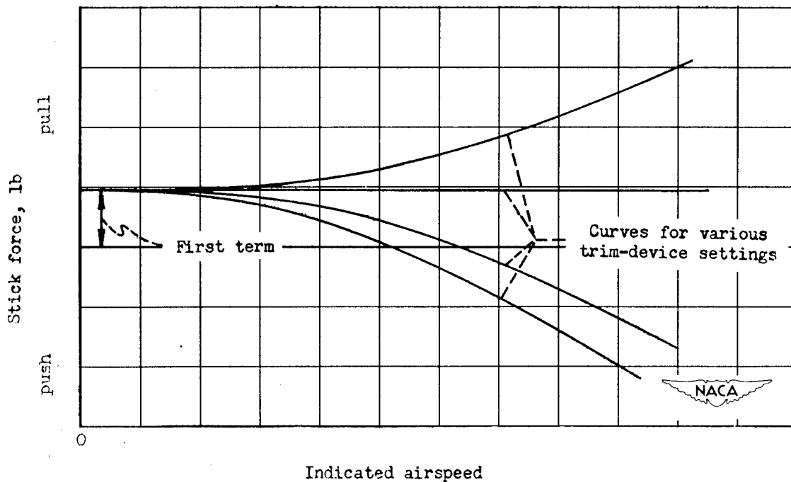
(b) Feel device, equation (4).
