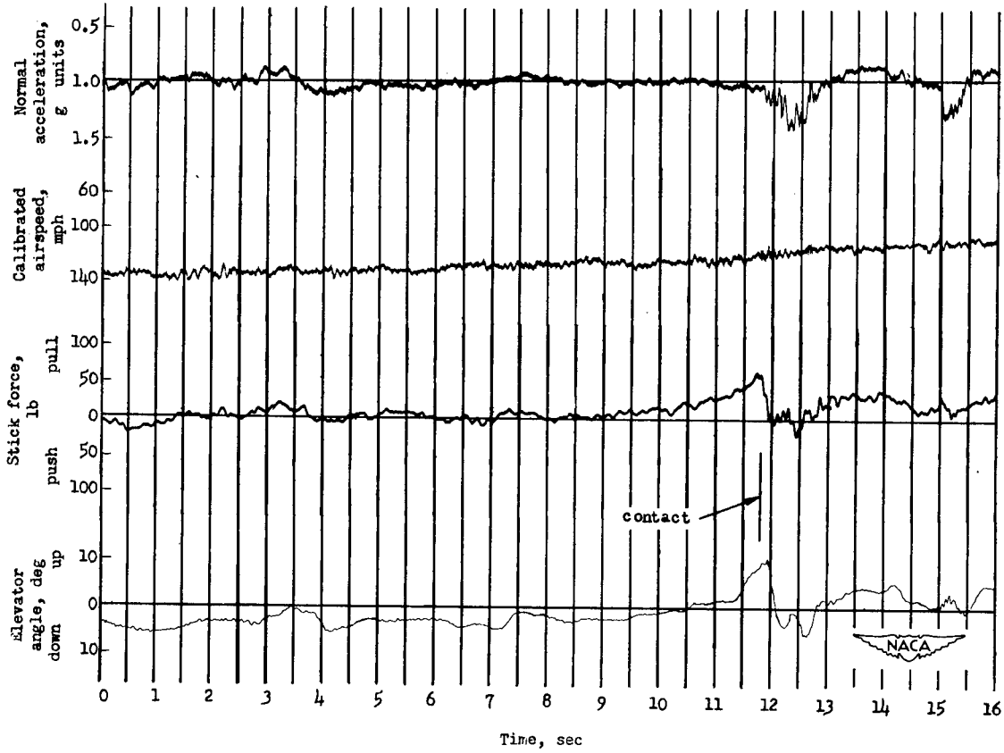
(c) Feel-device setting B.
