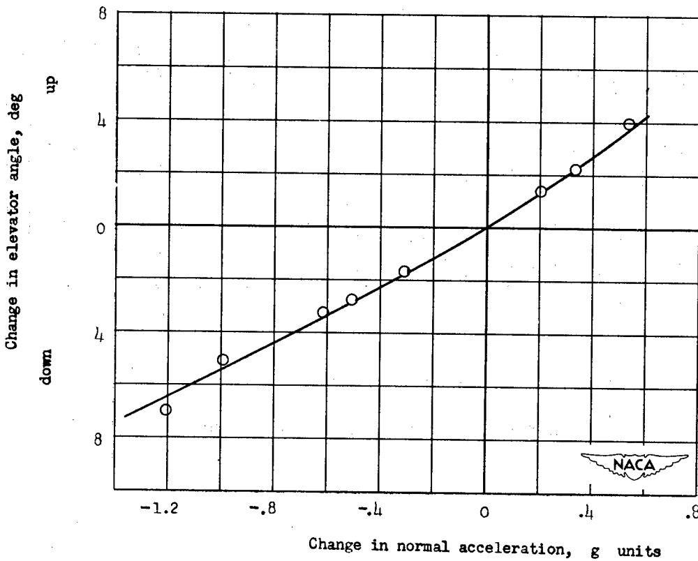
Figure 18.- Variation of stick force and elevator angle with normal acceleration for the airplane without the feel device in the approach condition showing elevator overbalance. Calculated feel-device forces shown for comparison.
