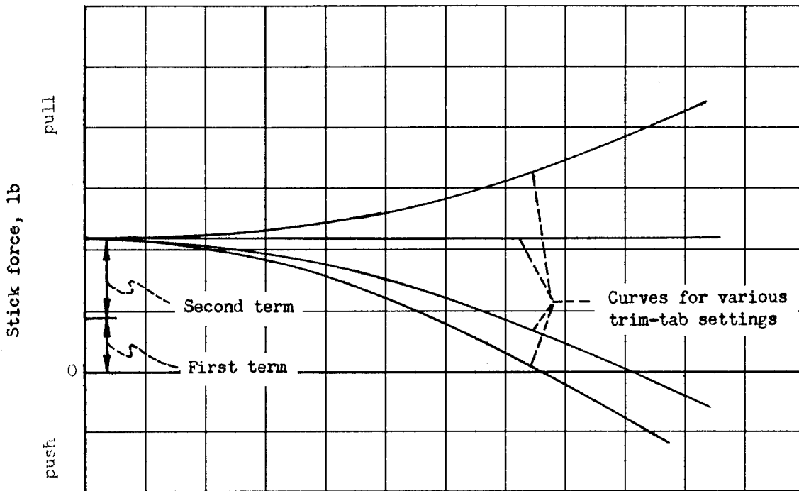
(a) Aerodynamic system, equation (3).
