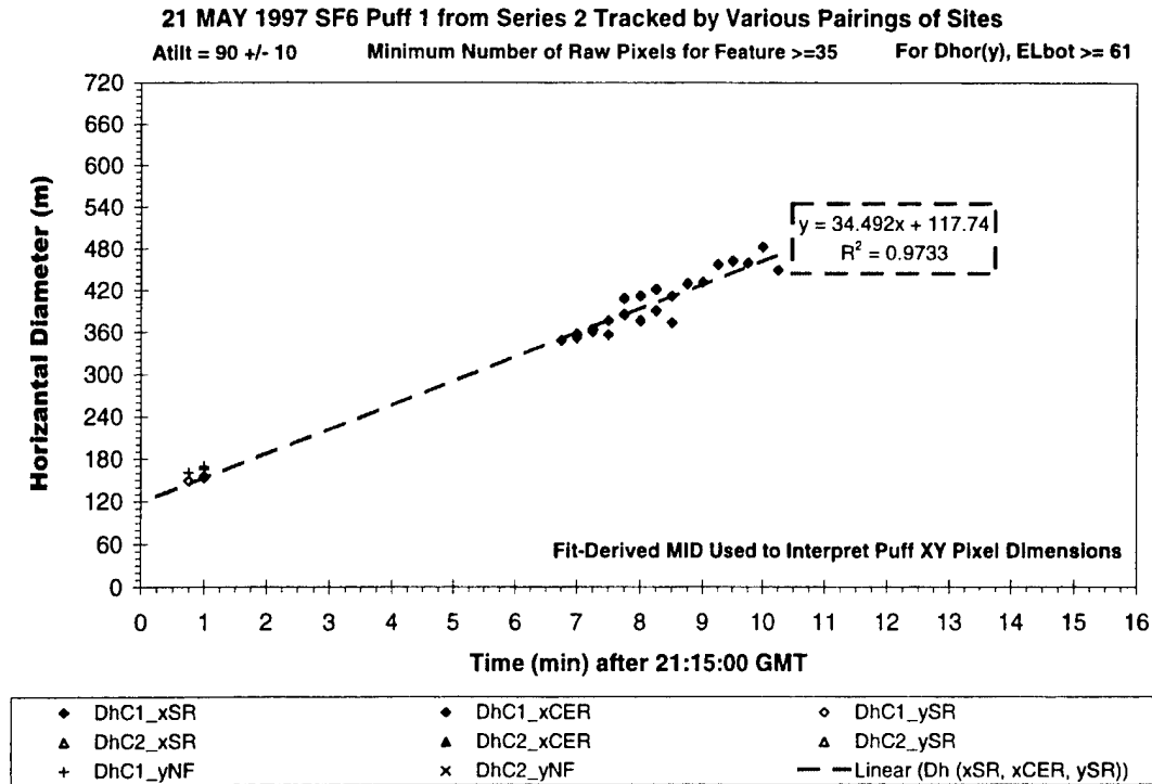
Figure G-7. "Best" crosswind extent versus time (expansion rate in m/min).
