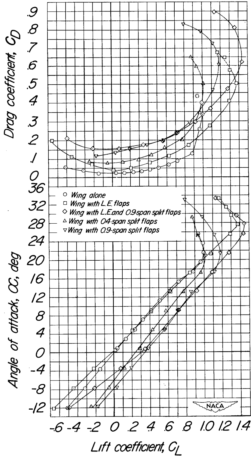
Figure 4.- Variation of angle of attack and drag coefficient with lift coefficient for various test configurations.
