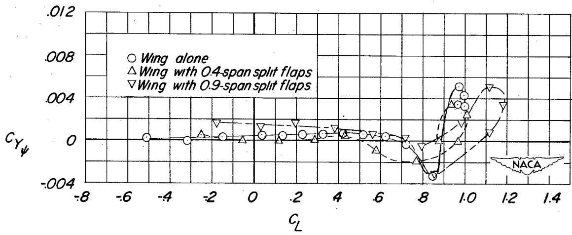
Figure 7.- Variation of C_{Y\psi} with lift coefficient for the various test configurations.
