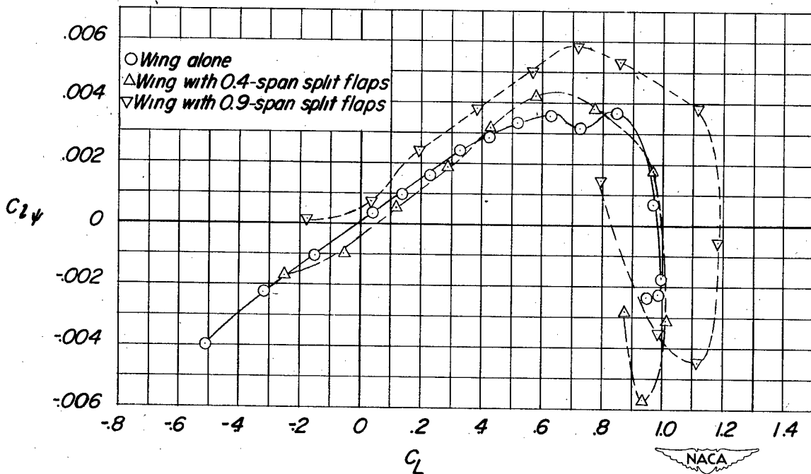
Figure 5- Variation of C_{l_{\psi}} with lift coefficient for the various test configurations.
