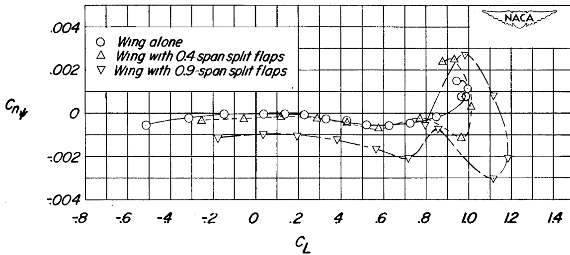
Figure 6- Variation of C_{n\psi} with lift coefficient for the various test configurations.
