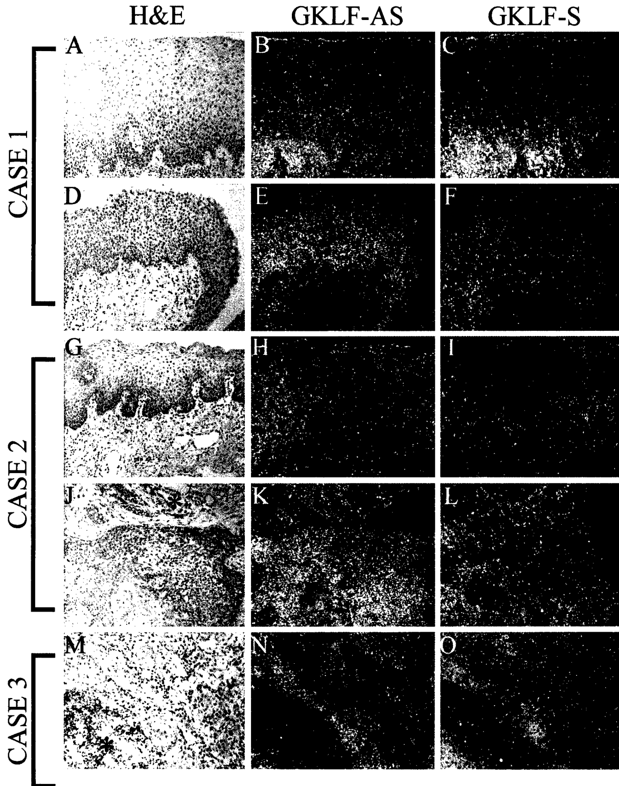
Fig. 5. ISH analysis of GKLf . Paraffin-embedded (A-L) or fresh-frozen (M-O) tissues were analyzed using antisense ( GKLf -AS) or sense ( GKLf -S) 35 S-labeled RNA probes. Each image (A-O) is 650 μm × 530 μm. Sections were stained with H&E. Case 1, A-C, uninvolved epithelium in a patient with primary laryngeal squamous cell carcinoma; D-F, adjacent dysplastic epithelium within the same tissue block. Case 2, G-I, uninvolved epithelium; J-L, adjacent primary tumor nests within stroma in the same tissue block; *, a salivary gland and ducts. Case 3, M-O, metastatic laryngeal squamous cell carcinoma infiltrating a lymph node; *, lymphocytes.
