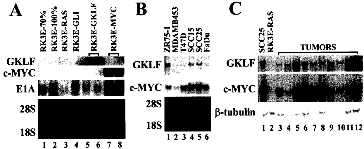
Fig. 3. Northern blot analysis of c-MYC and GKLF expression. Total RNA (25 \mu g) was loaded for each sample. A , analysis of transgene expression in RK3E cells and derivative cell lines transformed by the indicated oncogene. Lane 1, RK3E cells in exponential growth phase; Lane 2, RK3E cells incubated at confluence for 5 days. Ethidium bromide-stained RNA is shown below after transfer to the filter. B , endogenous GKLF (3.0 kb) or c-MYC (2.3 kb) expression in tumor cell lines. Lanes 1–3, breast cancer lines; Lanes 4–6, squamous cell carcinoma lines. C , analysis of gene expression in laryngeal squamous cell carcinoma. Lane 1, SCC25 cell line; Lanes 3–6, 9, and 12, primary tumors; Lanes 7, 8, 10, and 11, metastatic tumors; Lanes 3–12 correspond to case numbers 5, 8, 18–20, 6, and 21–24, respectively (see Table 4). RK3E-RAS cell RNA served as a negative control (Lane 2), whereas hybridization to \beta -tubulin served as a control for loading.
